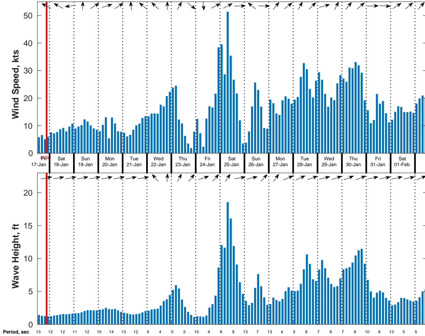
Wind & Wave Forecast for NDBC 62305 from 17-Jan-2025 12:00:00 to 02-Feb-2025 12:00:00
