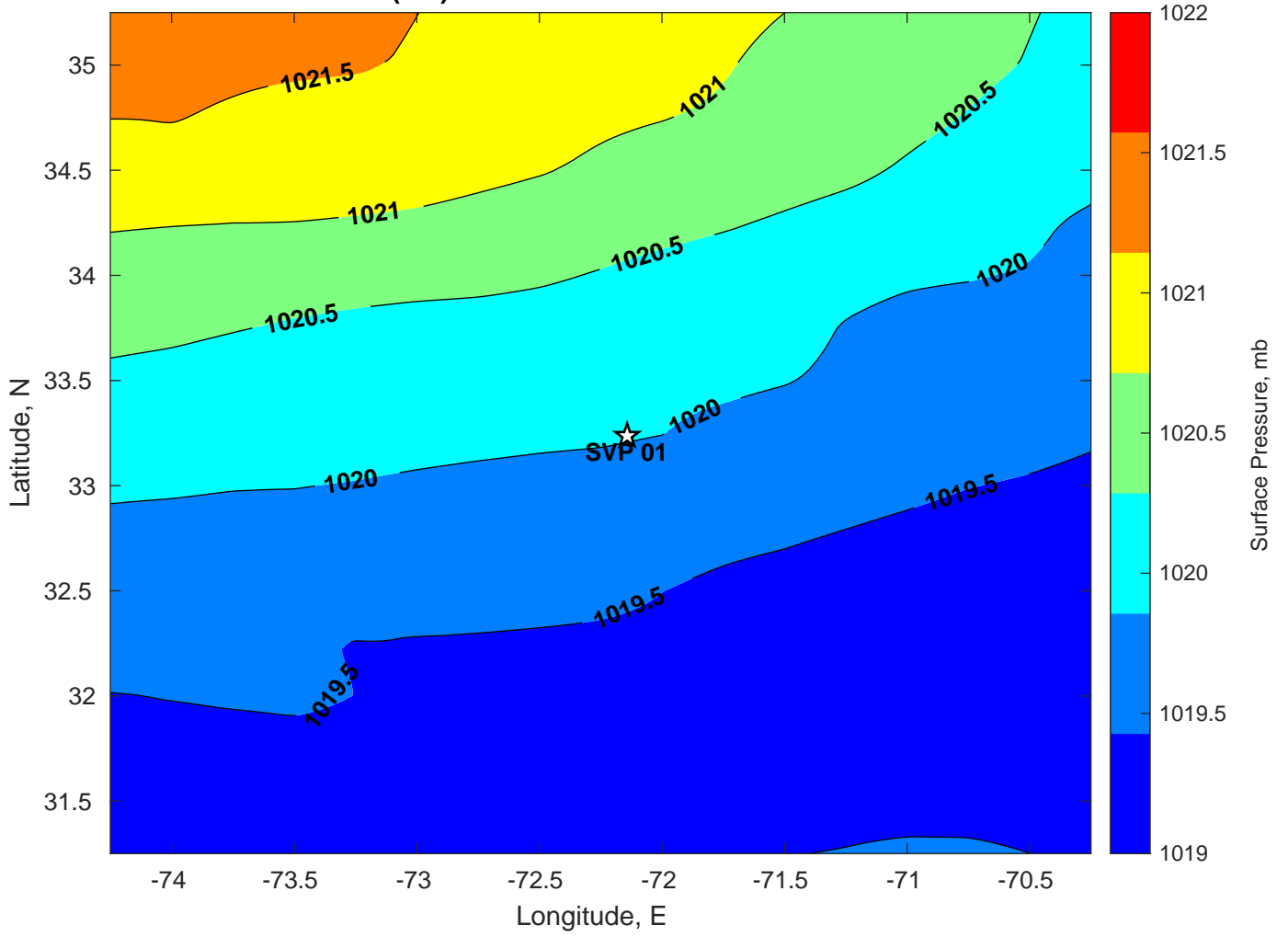
Surface Pressure (mb) for SVP 01 at 03-Jul-2024 00:00:00
