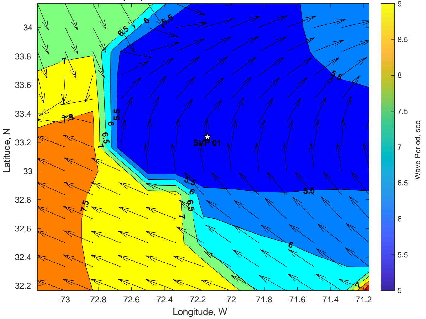
Wave Period (sec) for SVP 01 at 02-Jul-2024 06:00:00
