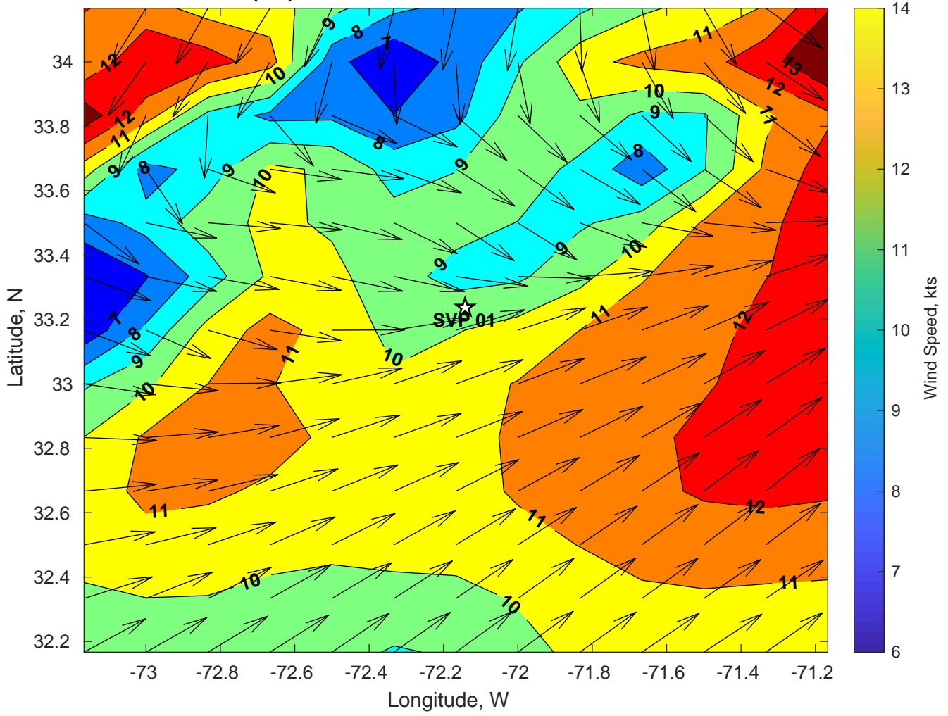
Winds (kts) for SVP 01 at 02-Jul-2024 06:00:00
