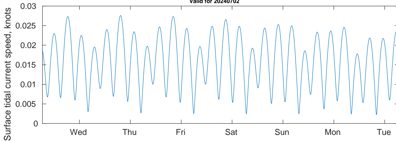
Tidal Currents and Heights for SVP 01 at 20240702
