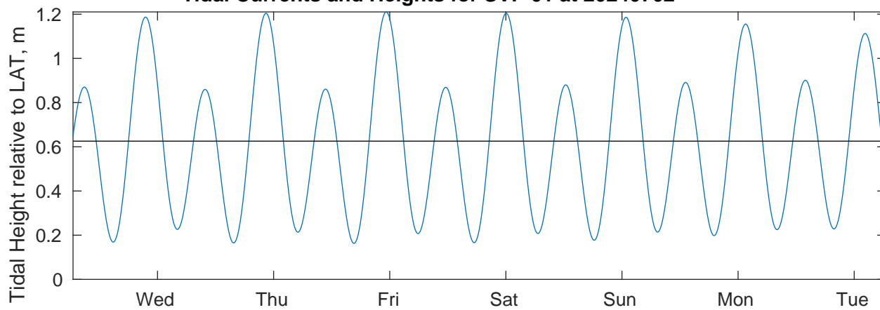
Tidal Currents and Heights for SVP 01 at 20240702
