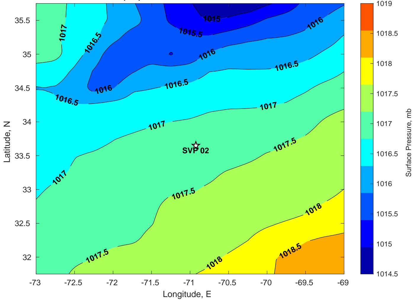
Surface Pressure (mb) for SVP 02 at 02-Jul-2024 00:00:00
