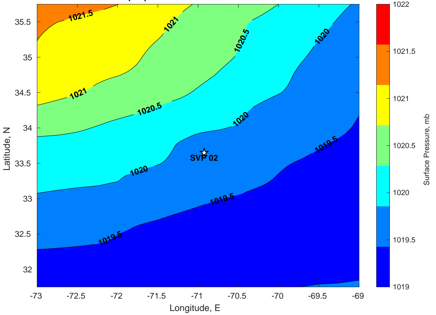
Surface Pressure (mb) for SVP 02 at 03-Jul-2024 00:00:00
