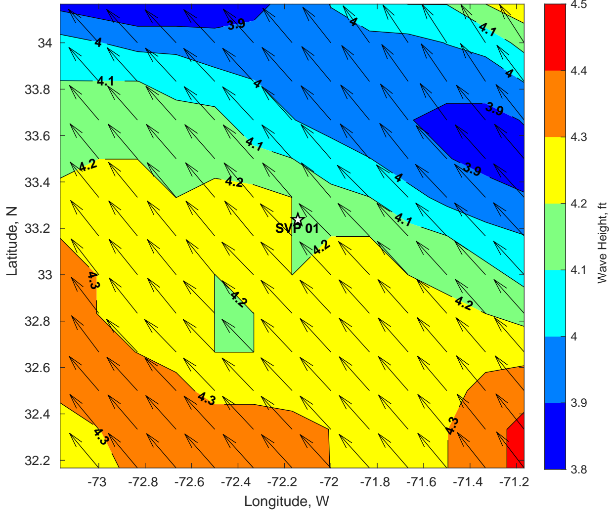
Wave Height (ft) for SVP 01 at 04-Jul-2024 06:00:00
