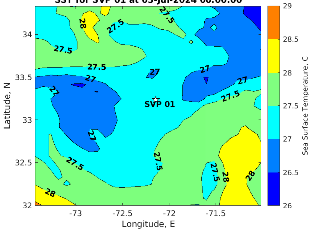
SST for SVP 01 at 03-Jul-2024 00:00:00
