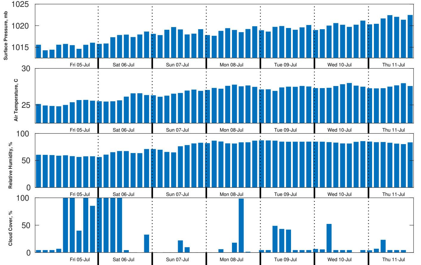
Met Forecast for SVP 01 from 05-Jul-2024 00:00:00 to 12-Jul-2024 00:00:00
