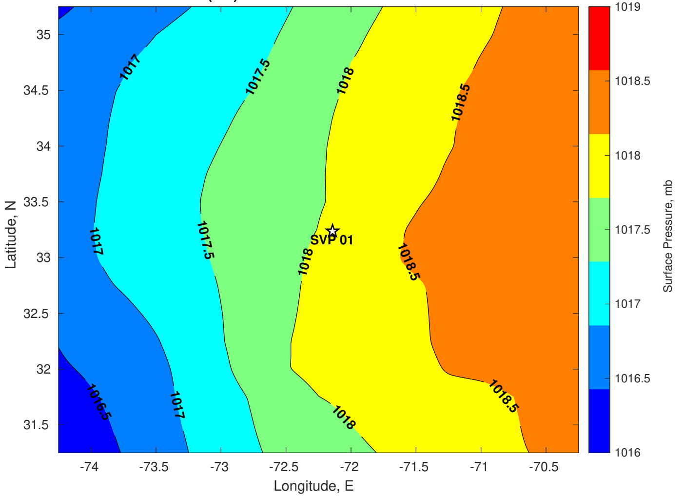
Surface Pressure (mb) for SVP 01 at 07-Jul-2024 00:00:00
