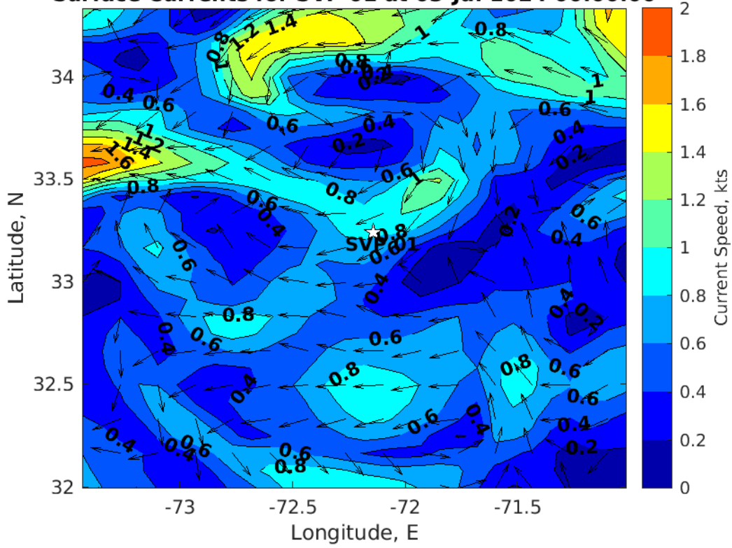
Surface Currents for SVP 01 at 03-Jul-2024 00:00:00
