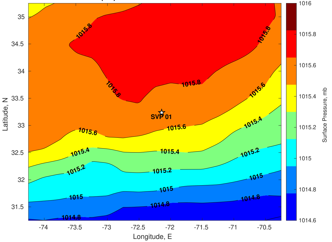
Surface Pressure (mb) for SVP 01 at 05-Jul-2024 00:00:00
