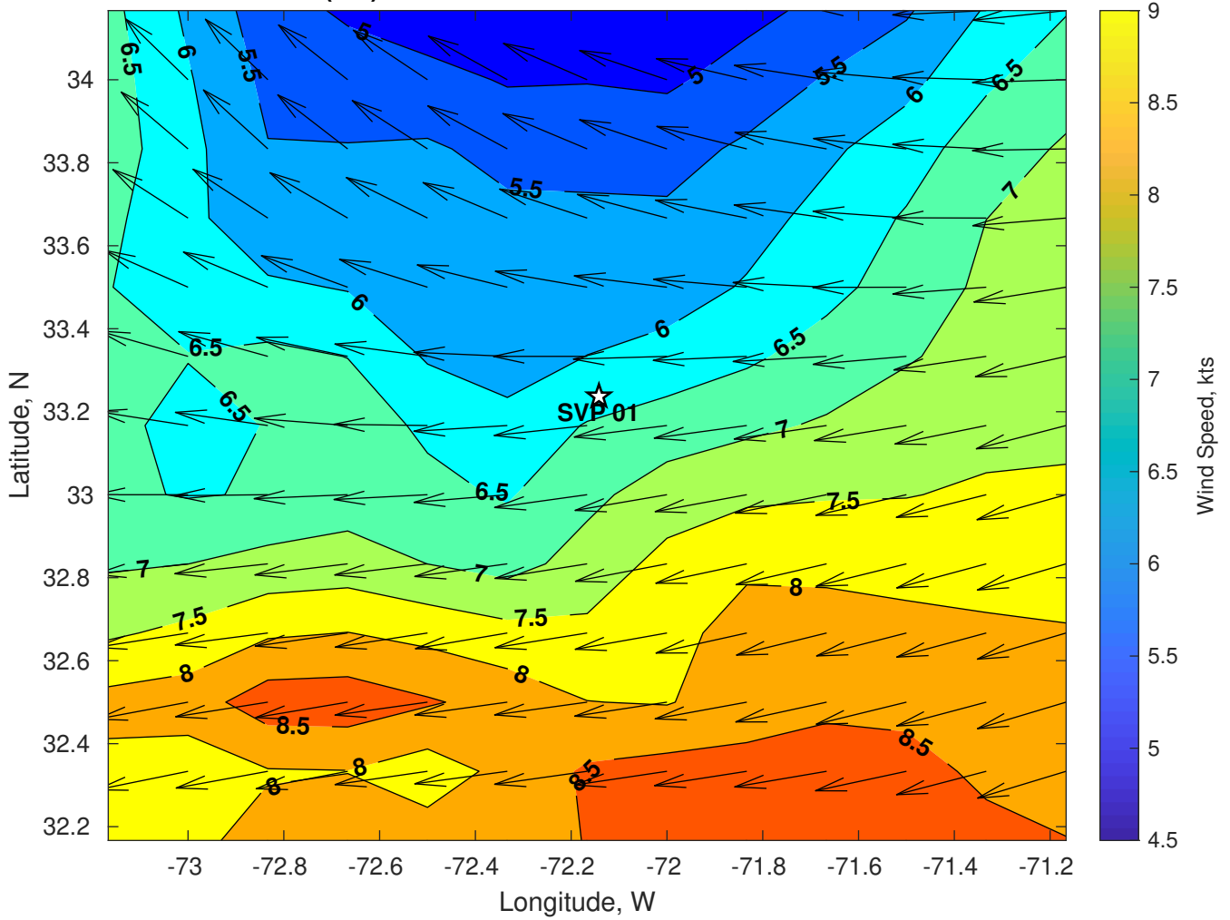
Winds (kts) for SVP 01 at 05-Jul-2024 06:00:00
