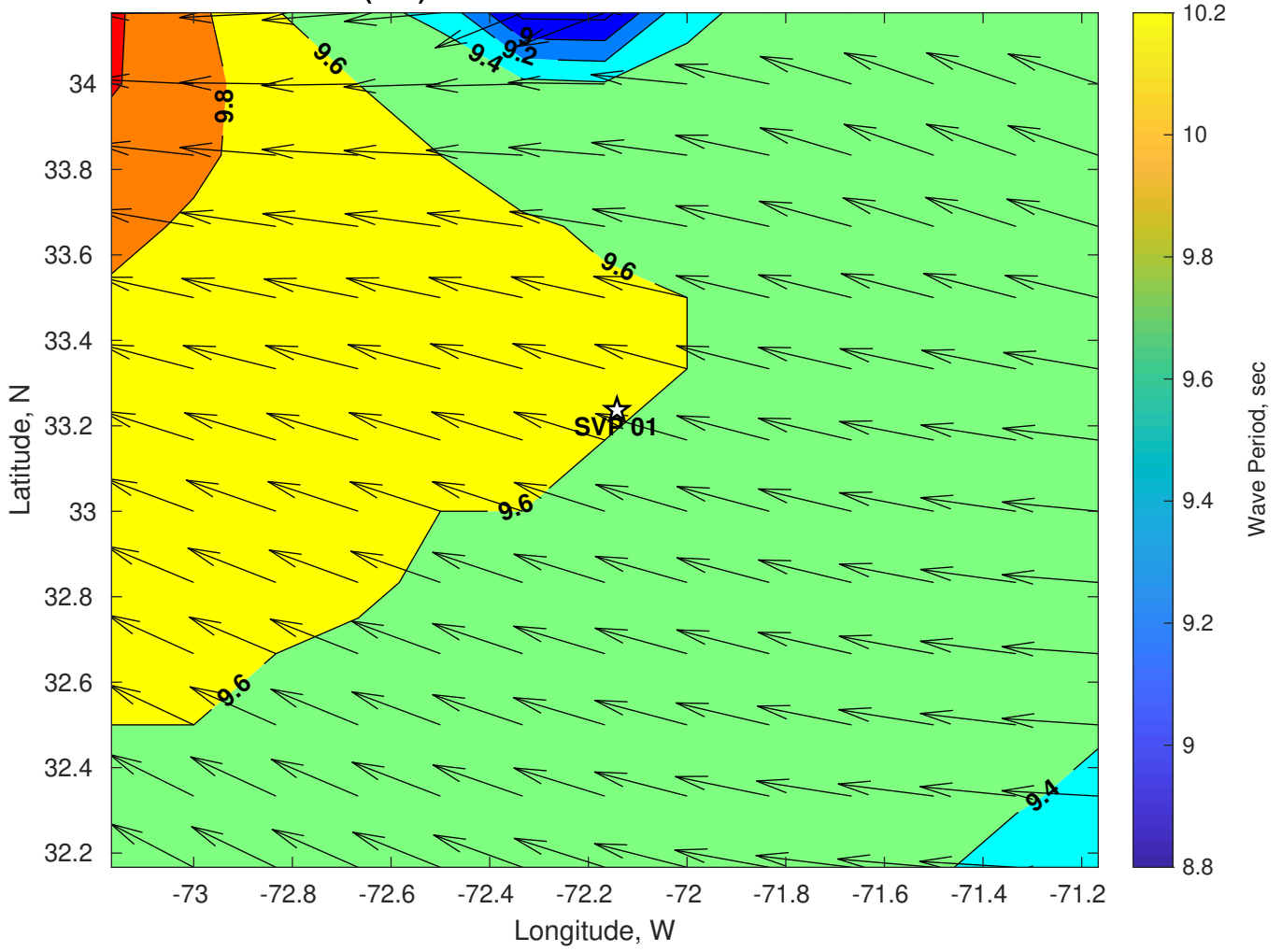
Wave Period (sec) for SVP 01 at 05-Jul-2024 06:00:00
