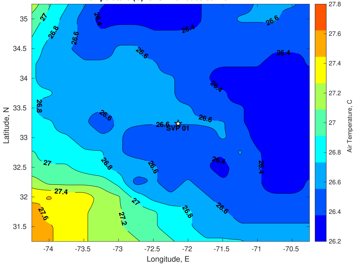
Air Temperature (C) for SVP 01 at 05-Jul-2024
