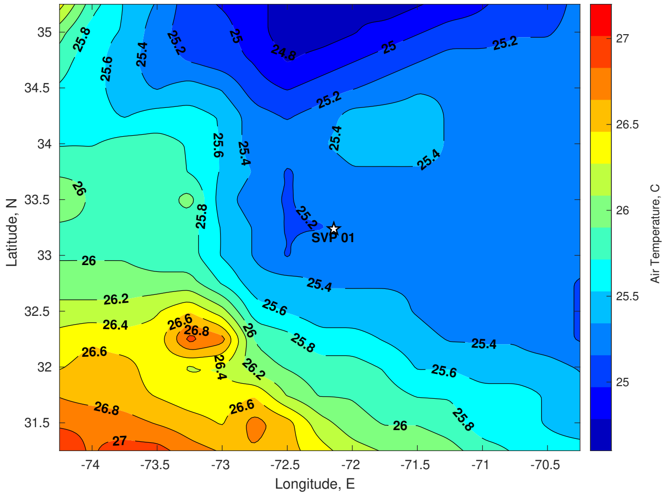
Air Temperature (C) for SVP 01 at 05-Jul-2024
