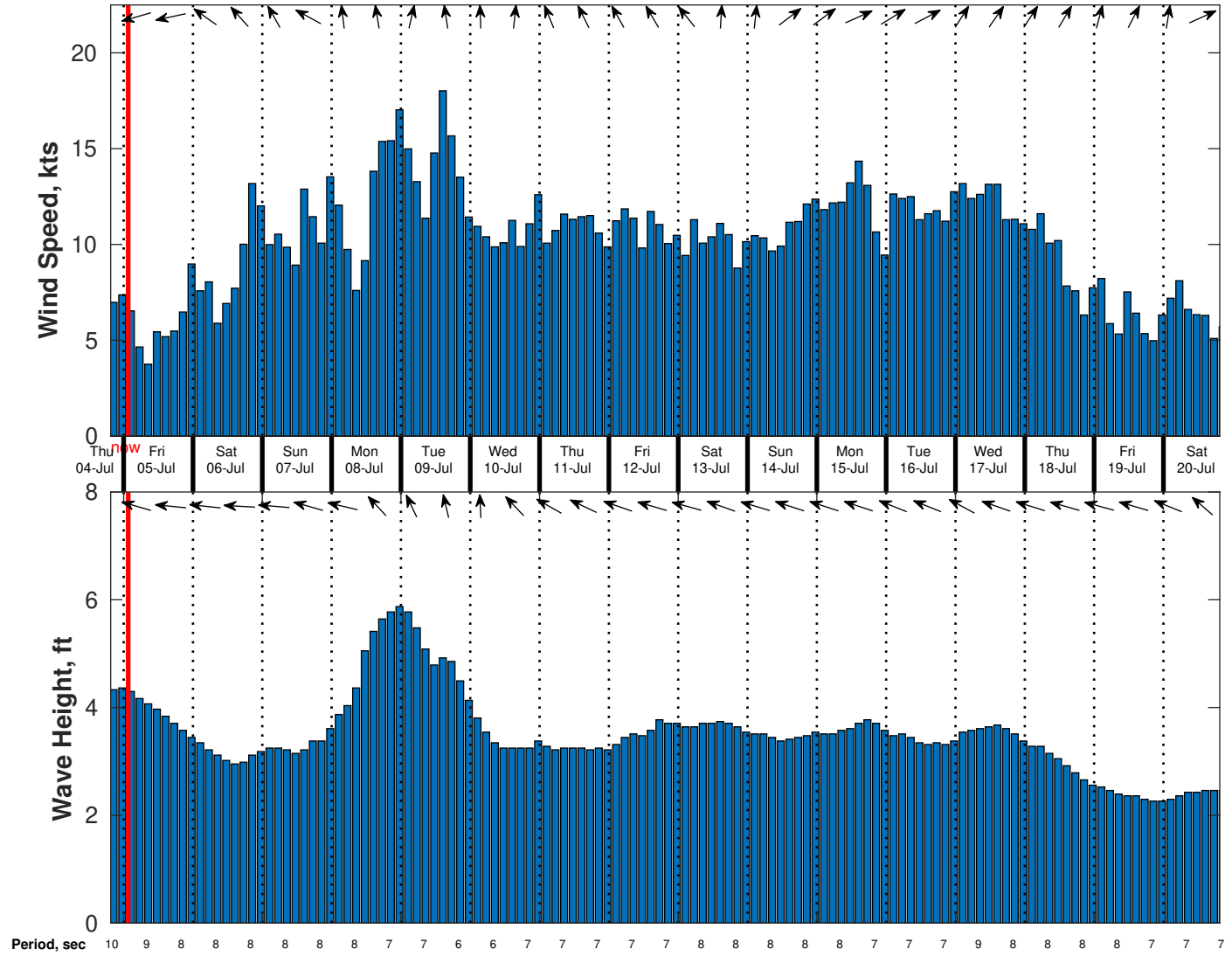
Wind & Wave Forecast for SVP 01 from 04-Jul-2024 19:00:00 to 20-Jul-2024 19:00:00
