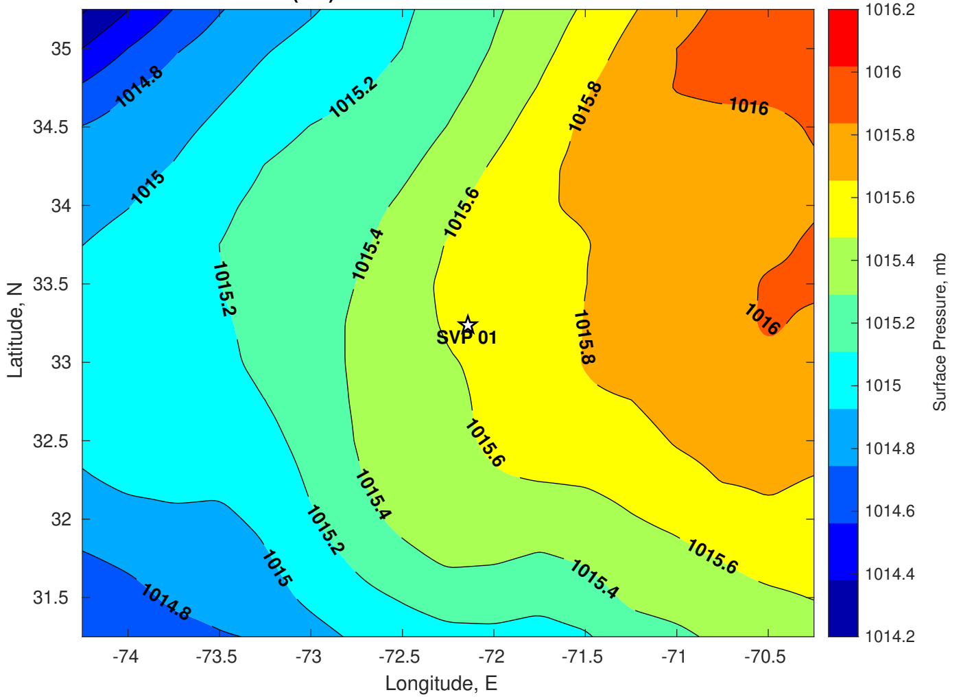
Surface Pressure (mb) for SVP 01 at 06-Jul-2024 00:00:00
