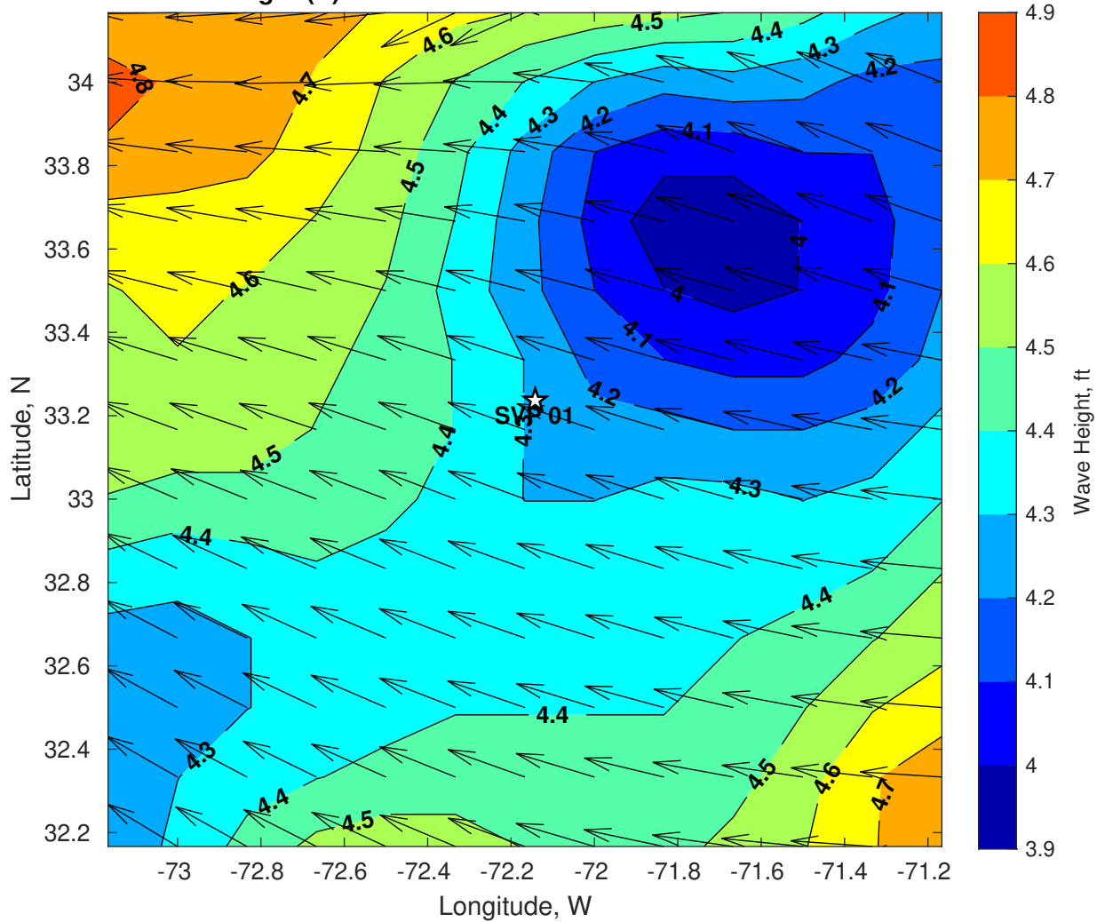
Wave Height (ft) for SVP 01 at 05-Jul-2024 06:00:00
