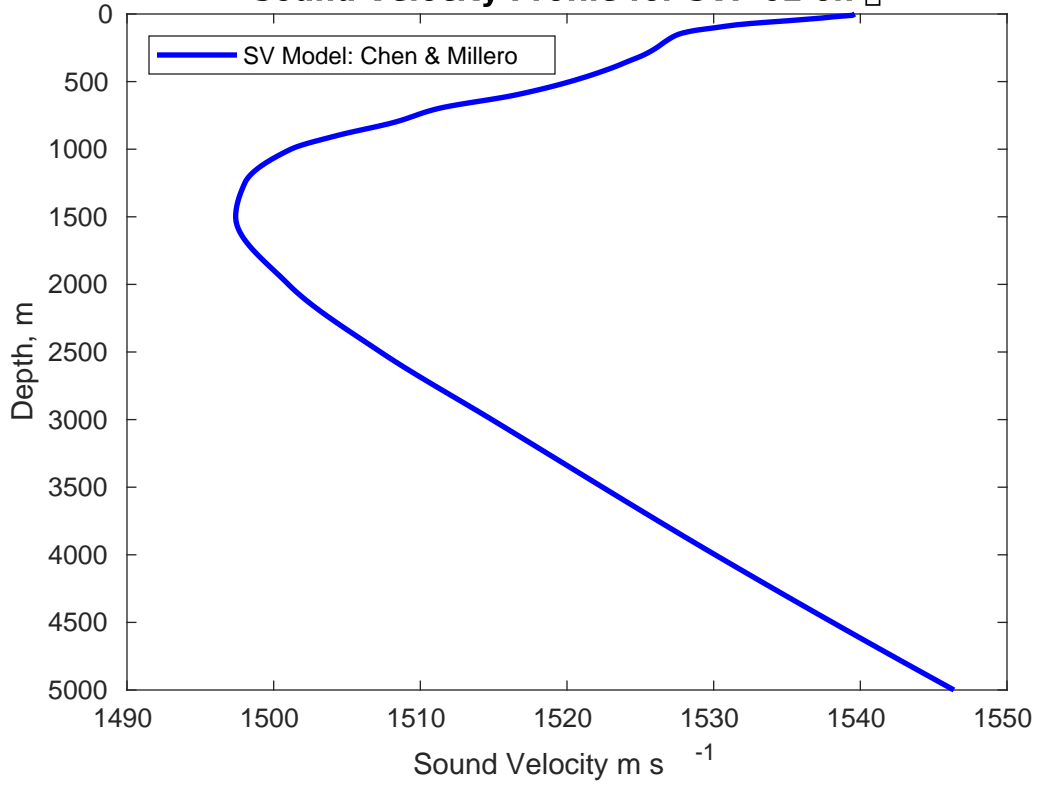
Sound Velocity Profile for SVP 02 on [ ]
