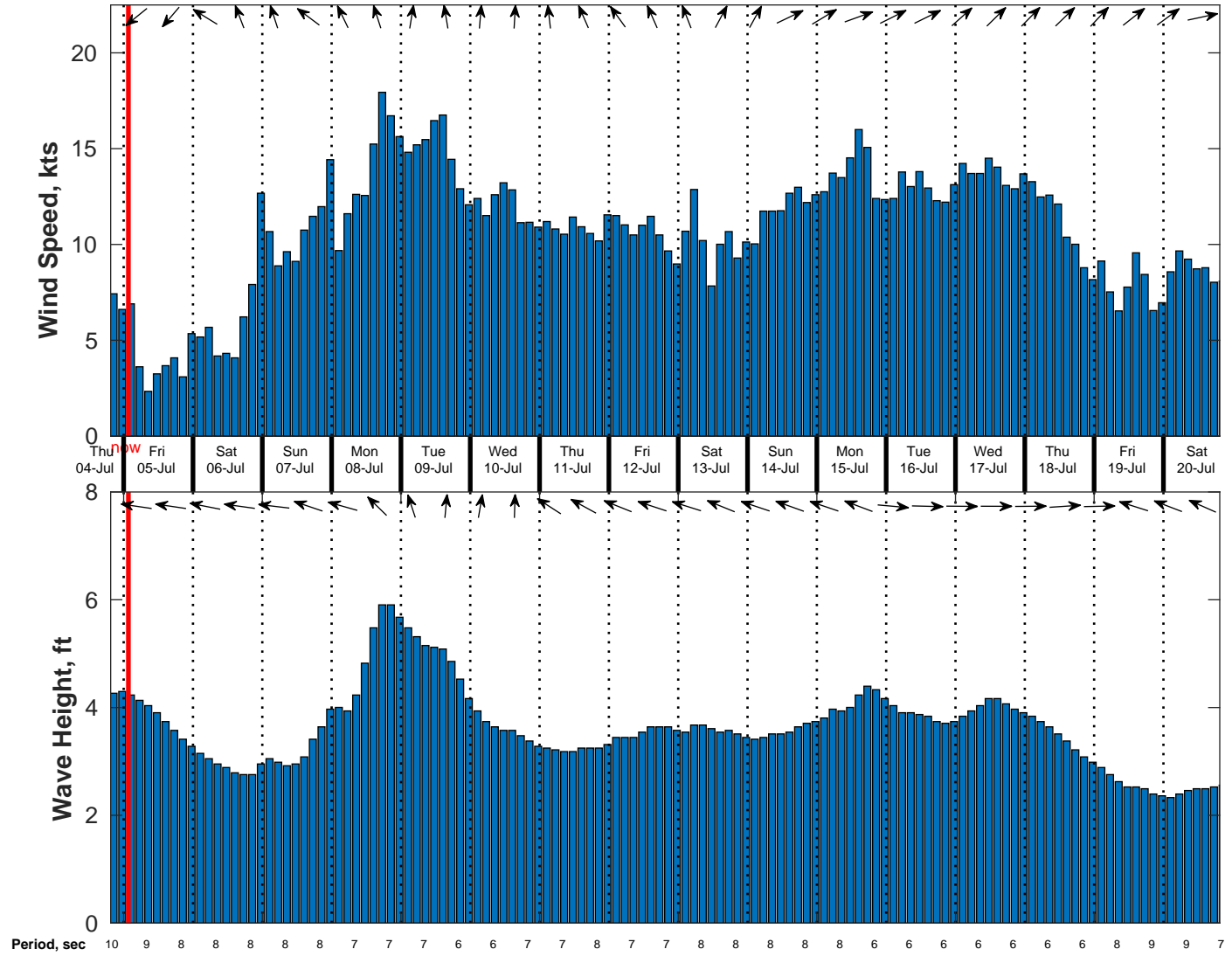
Wind & Wave Forecast for SVP 02 from 04-Jul-2024 19:00:00 to 20-Jul-2024 19:00:00
