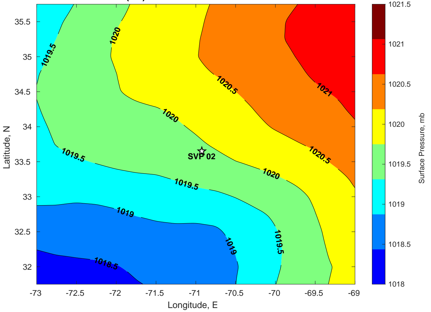
Surface Pressure (mb) for SVP 02 at 08-Jul-2024 00:00:00
