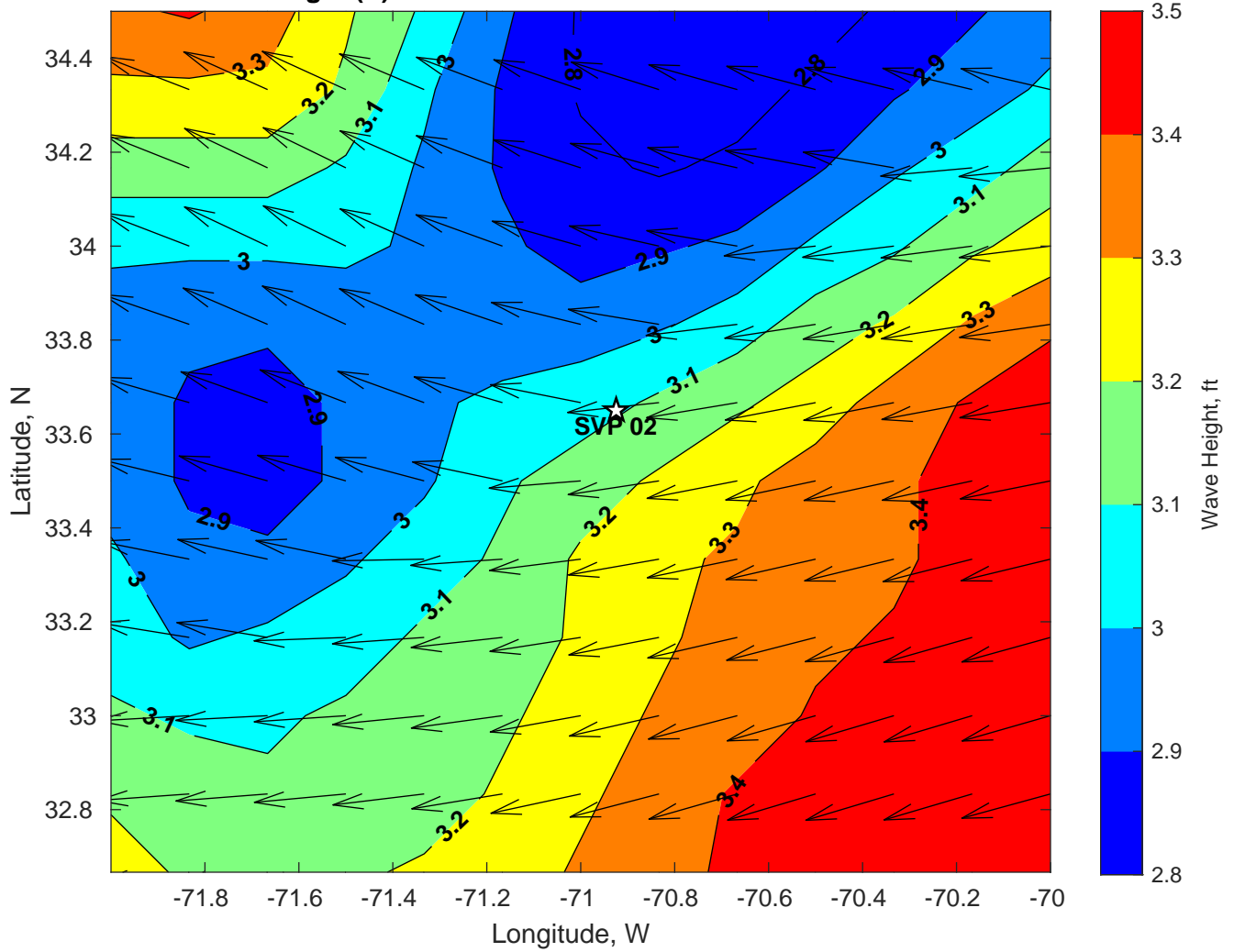
Wave Height (ft) for SVP 02 at 06-Jul-2024 06:00:00
