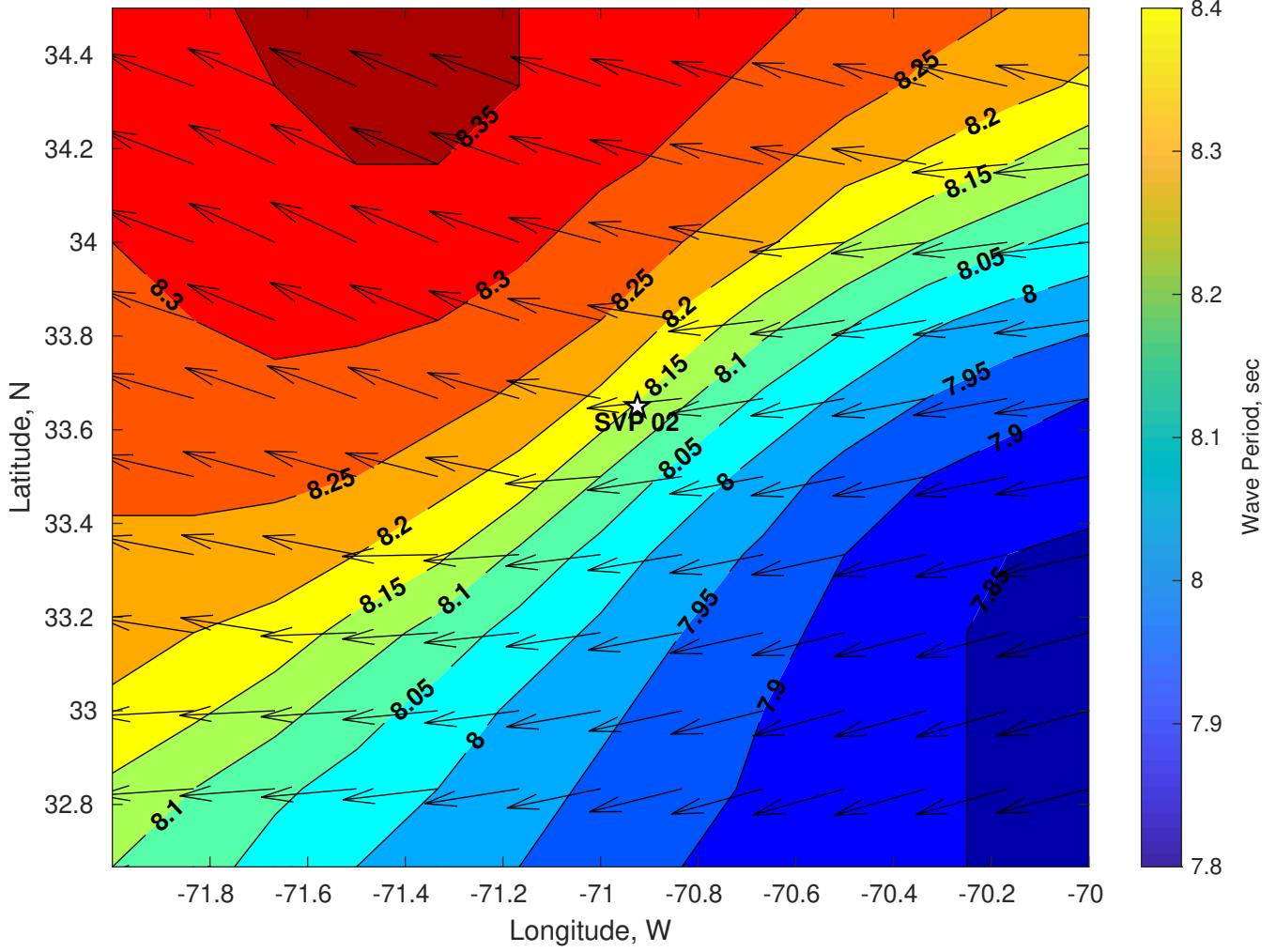
Wave Period (sec) for SVP 02 at 06-Jul-2024 06:00:00
