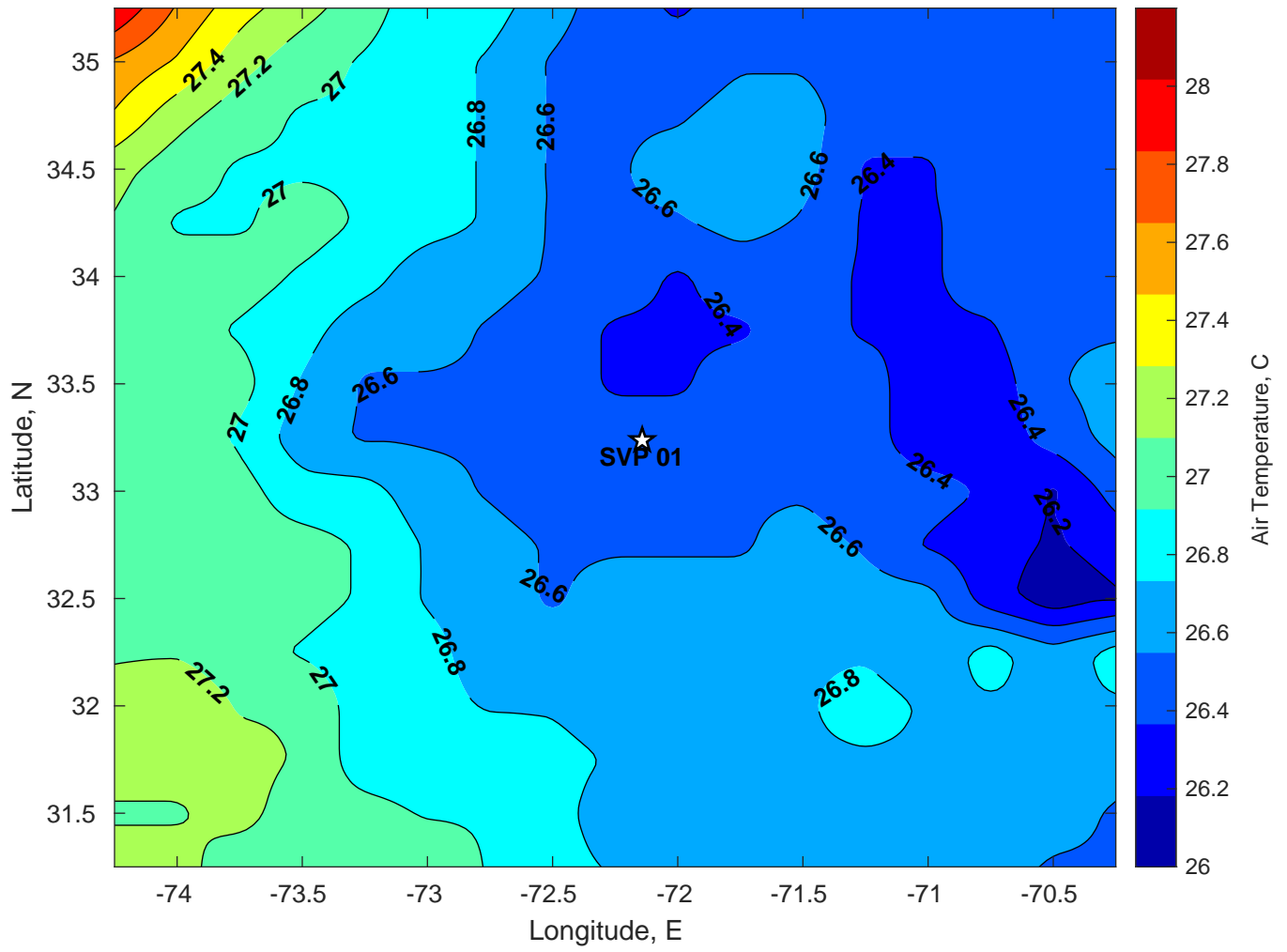
Air Temperature (C) for SVP 01 at 07-Jul-2024
