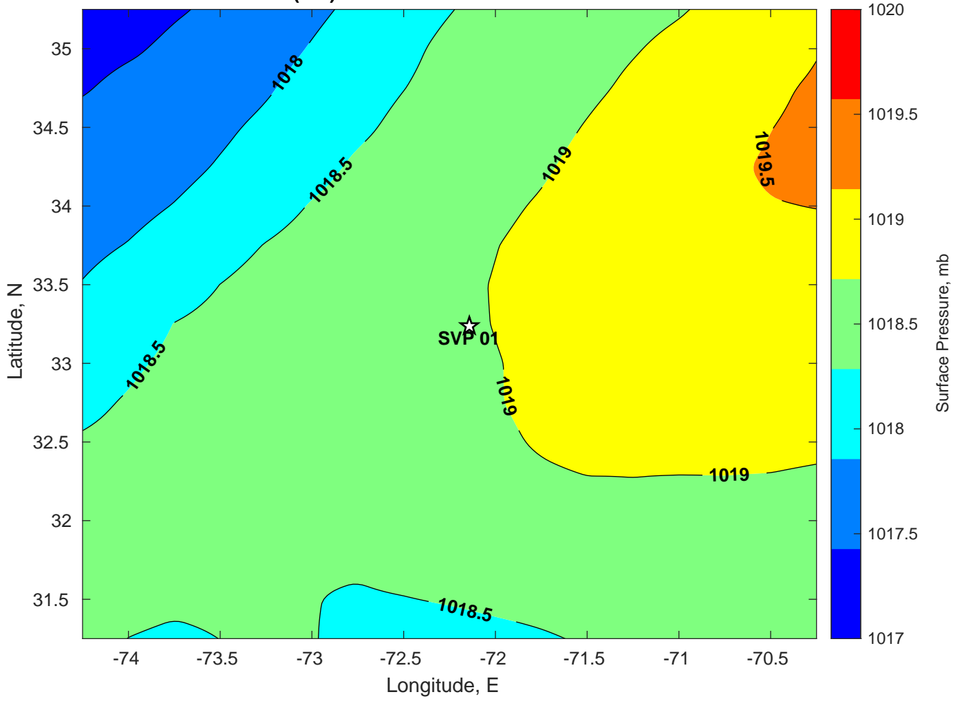
Surface Pressure (mb) for SVP 01 at 08-Jul-2024 00:00:00
