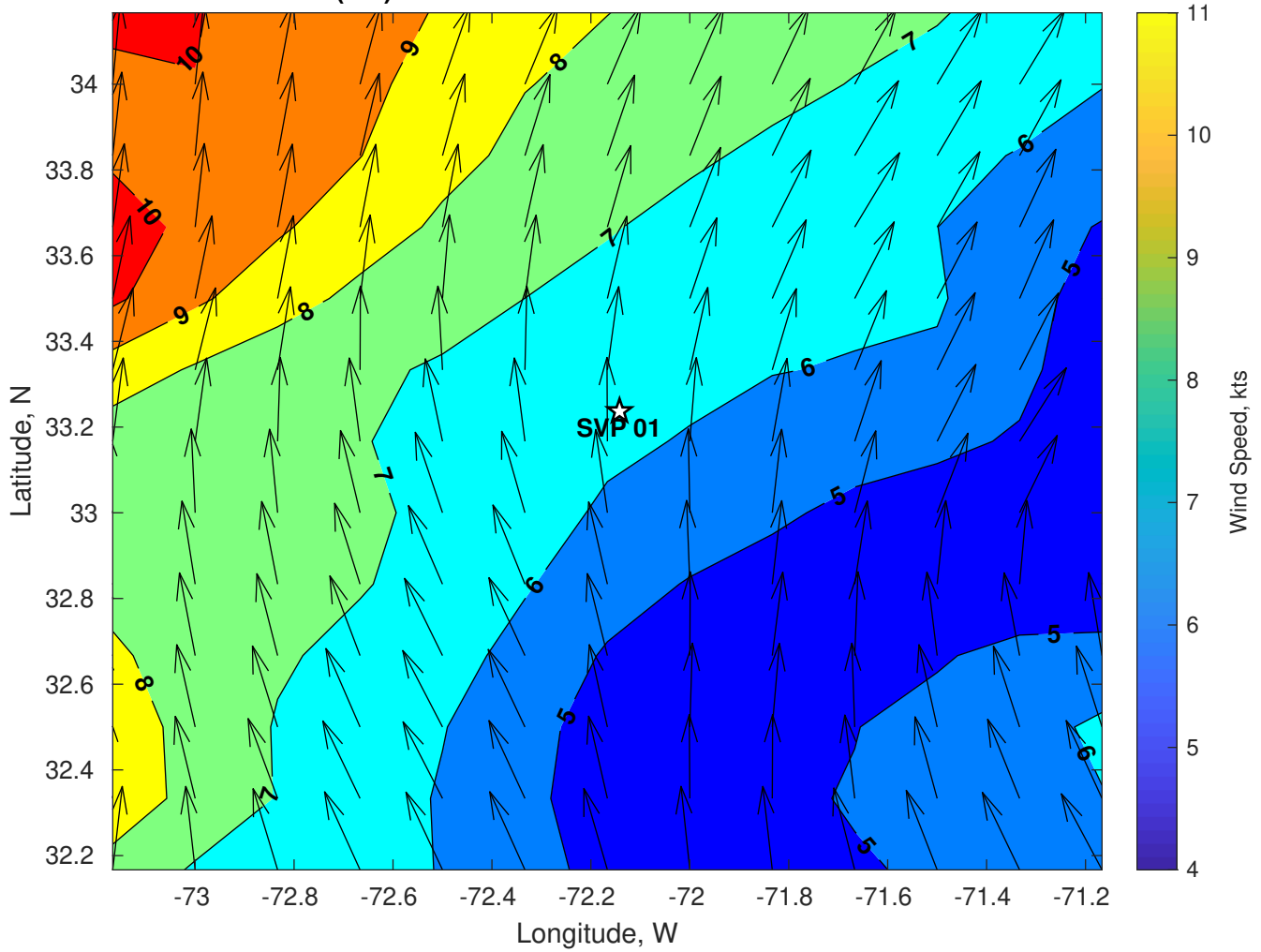
Winds (kts) for SVP 01 at 07-Jul-2024 06:00:00
