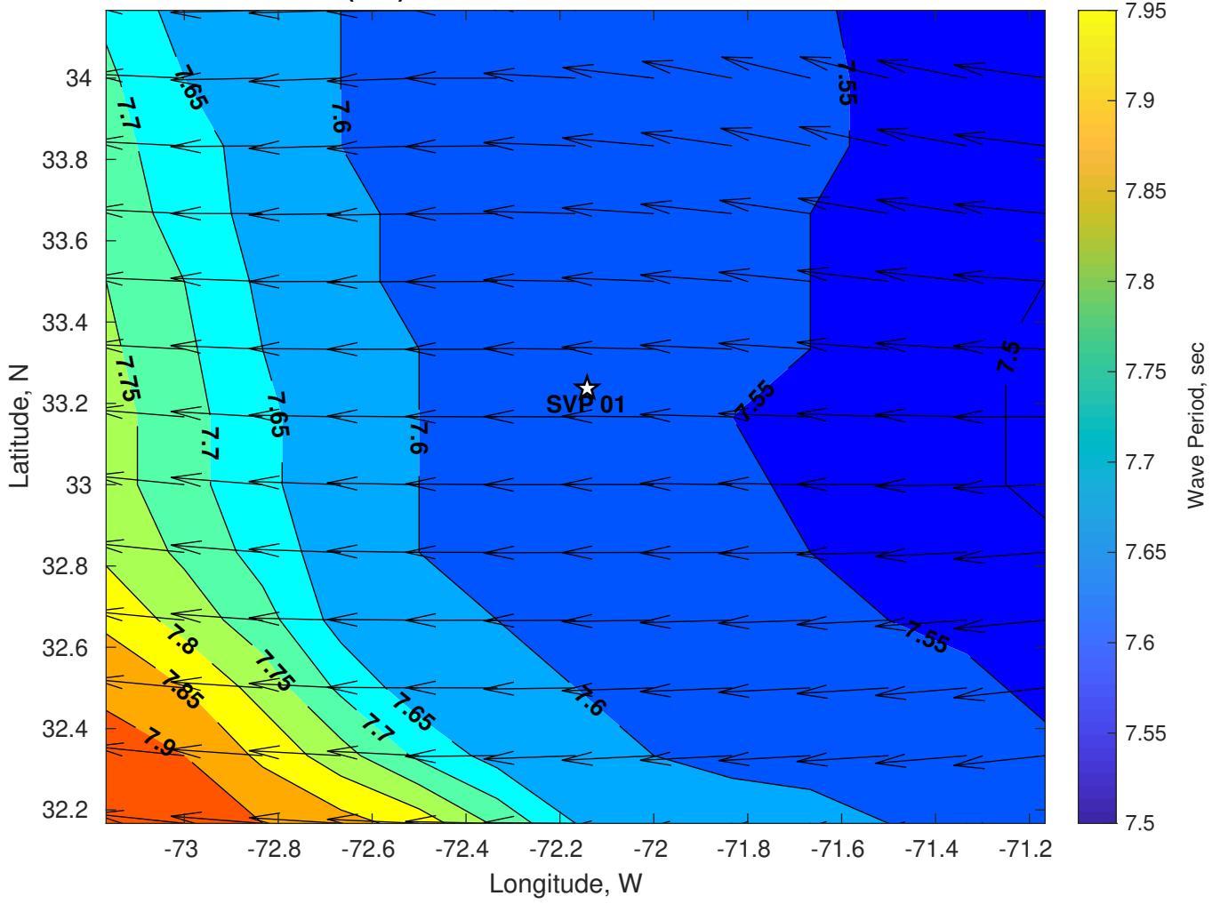
Wave Period (sec) for SVP 01 at 07-Jul-2024 06:00:00
