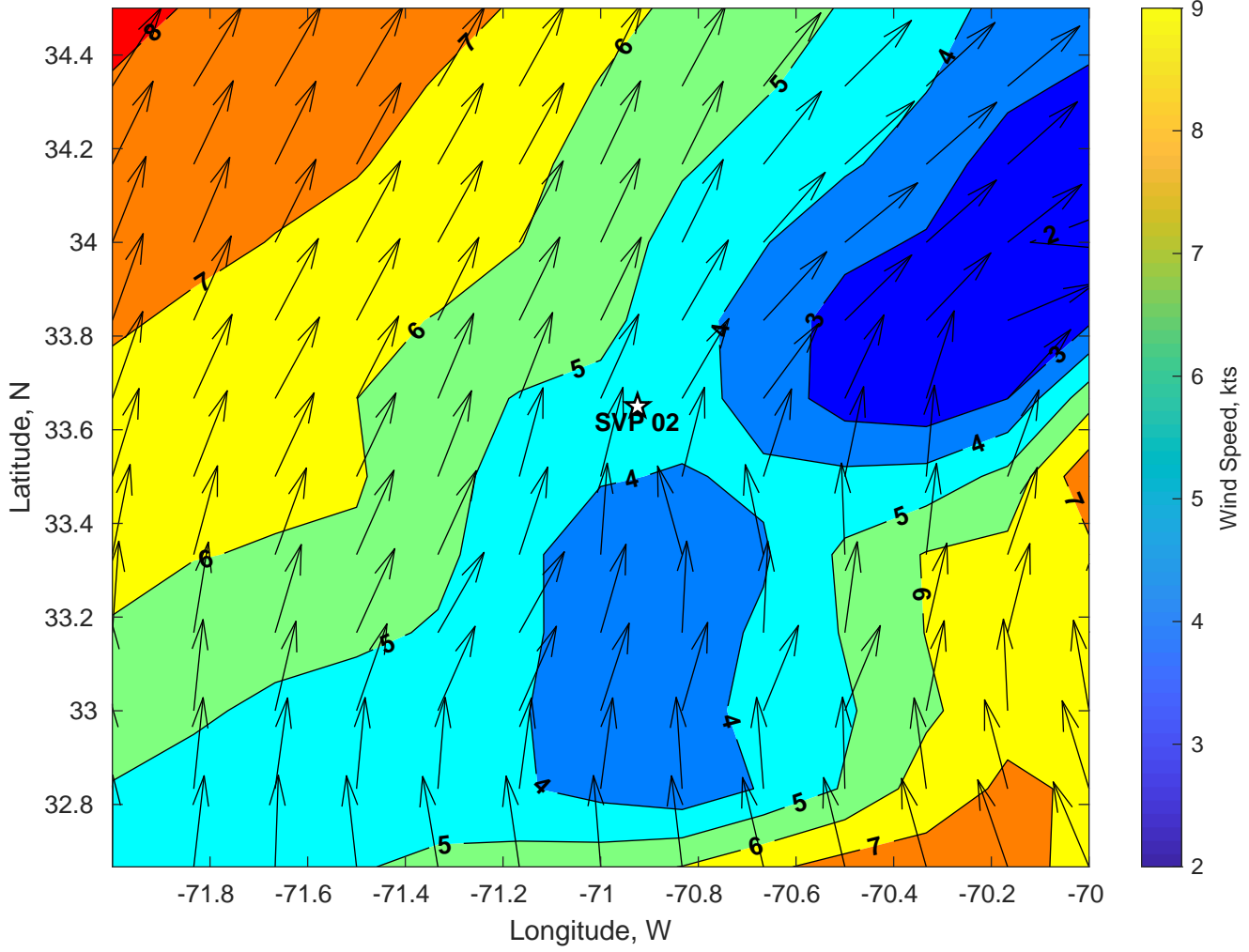
Winds (kts) for SVP 02 at 07-Jul-2024 06:00:00
