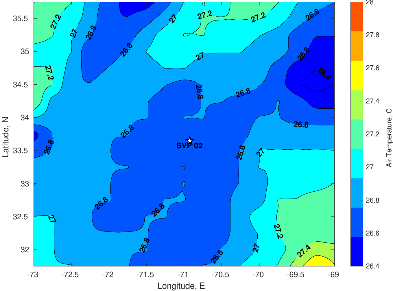
Air Temperature (C) for SVP 02 at 07-Jul-2024
