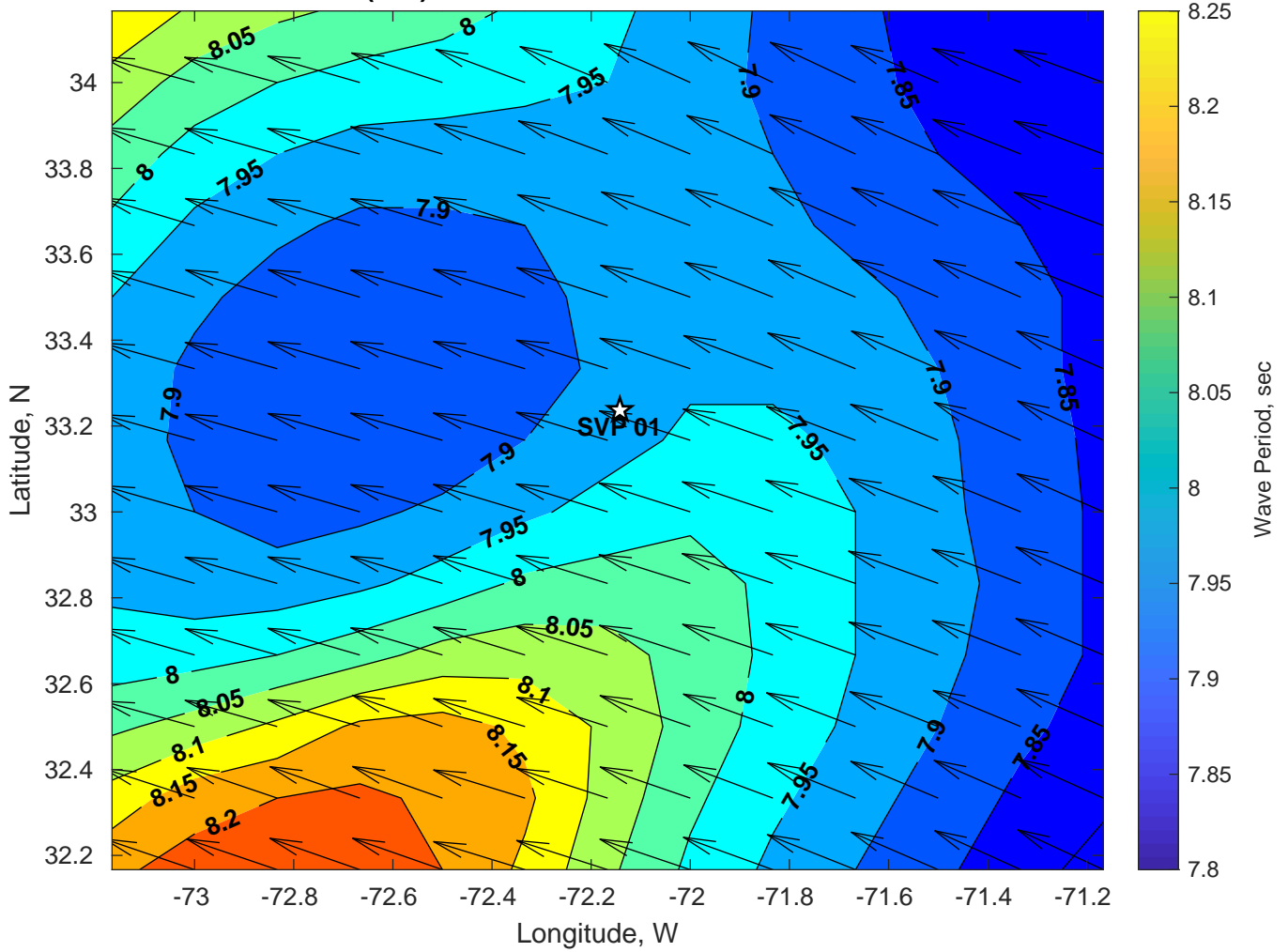
Wave Period (sec) for SVP 01 at 08-Jul-2024 06:00:00
