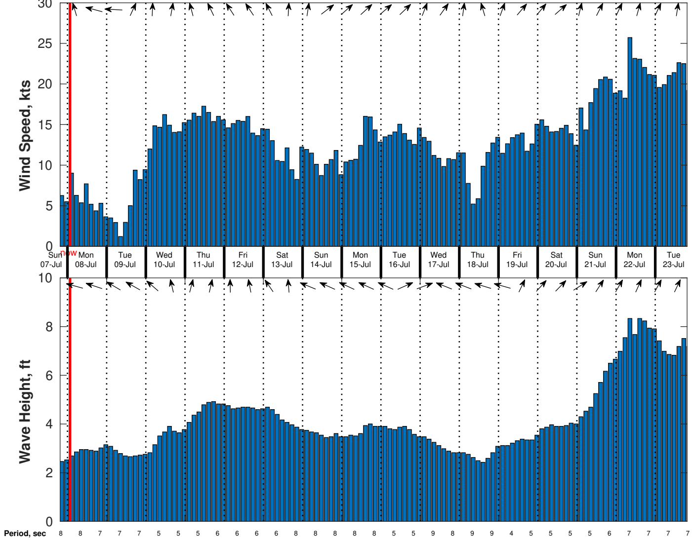
Wind & Wave Forecast for SVP 01 from 07-Jul-2024 19:00:00 to 23-Jul-2024 19:00:00
