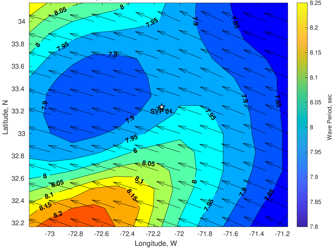
Wave Period (sec) for SVP 01 at 08-Jul-2024 06:00:00
