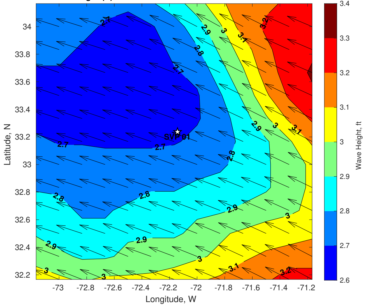
Wave Height (ft) for SVP 01 at 08-Jul-2024 06:00:00
