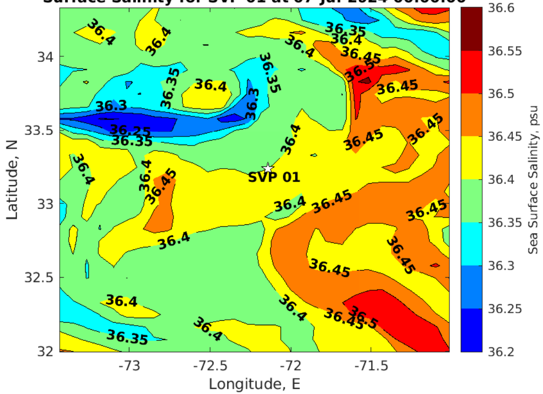
Surface Salinity for SVP 01 at 07-Jul-2024 00:00:00
