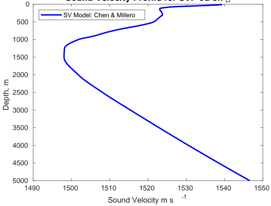
Sound Velocity Profile for SVP 01 on □
