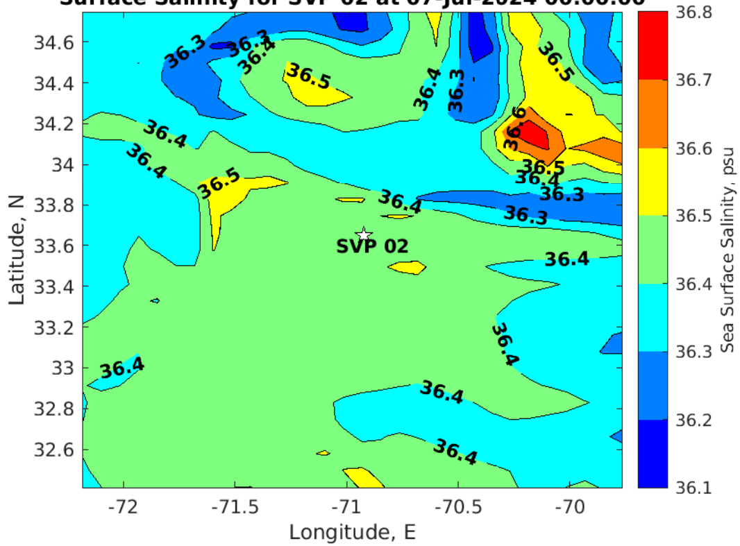
Surface Salinity for SVP 02 at 07-Jul-2024 00:00:00
