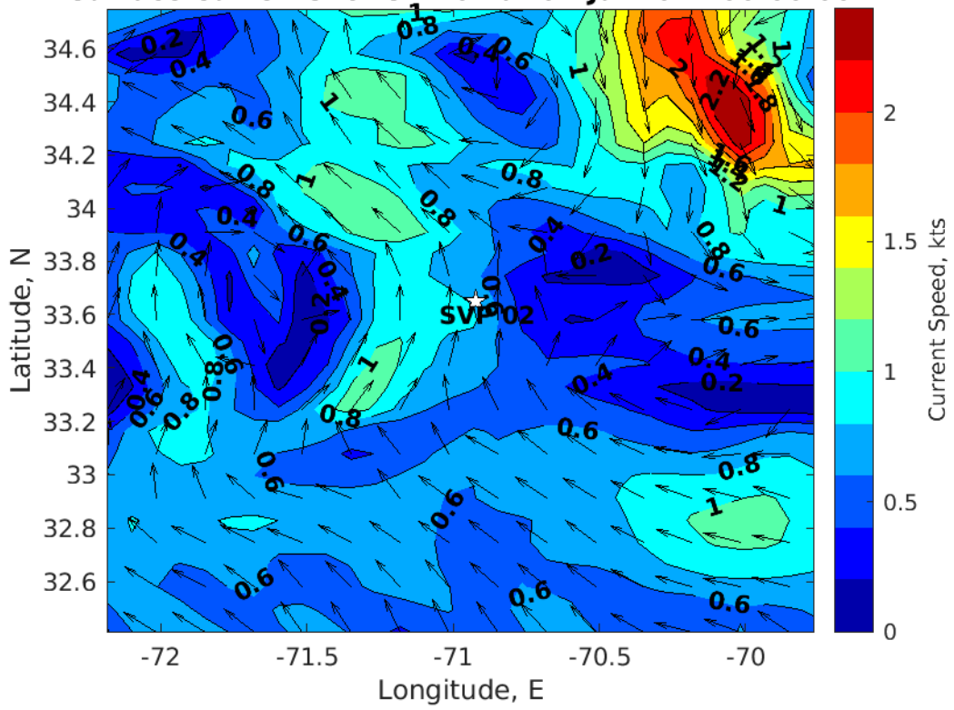
Surface Currents for SVP 02 at 07-Jul-2024 00:00:00
