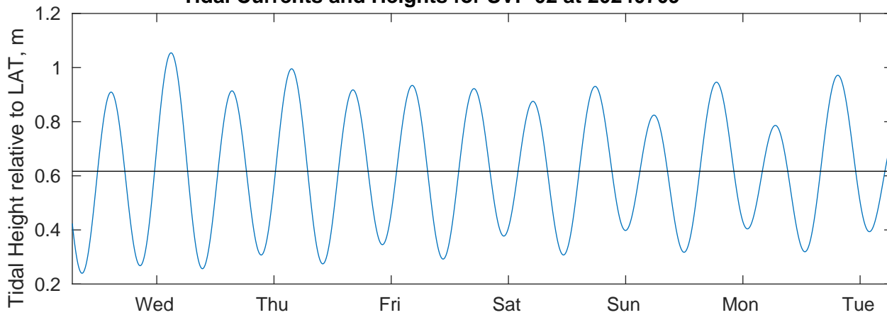
Tidal Currents and Heights for SVP 02 at 20240709
