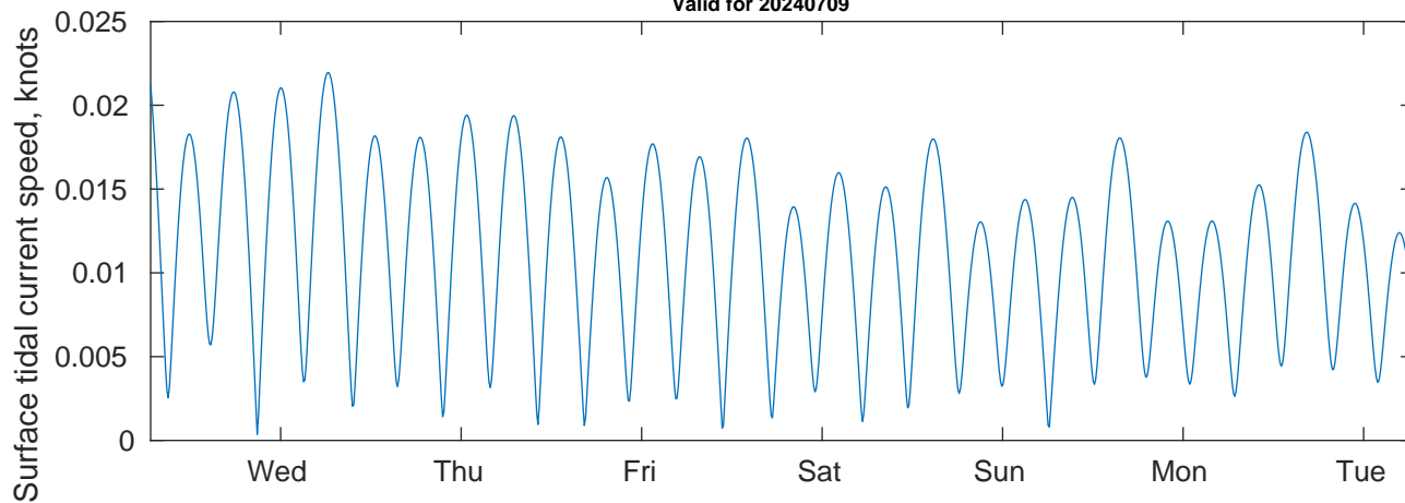
Tidal Currents and Heights for SVP 02 at 20240709
