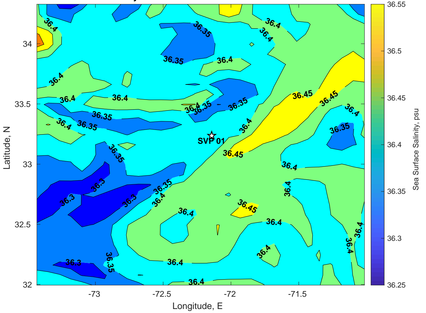
Surface Salinity for SVP 01 at 10-Jul-2024 00:00:00
