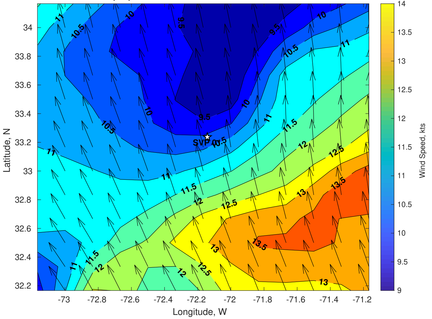
Winds (kts) for SVP 01 at 10-Jul-2024 06:00:00
