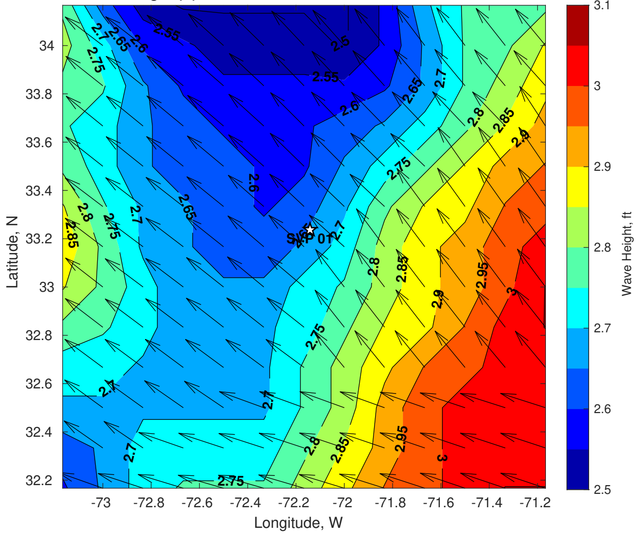
Wave Height (ft) for SVP 01 at 10-Jul-2024 06:00:00
