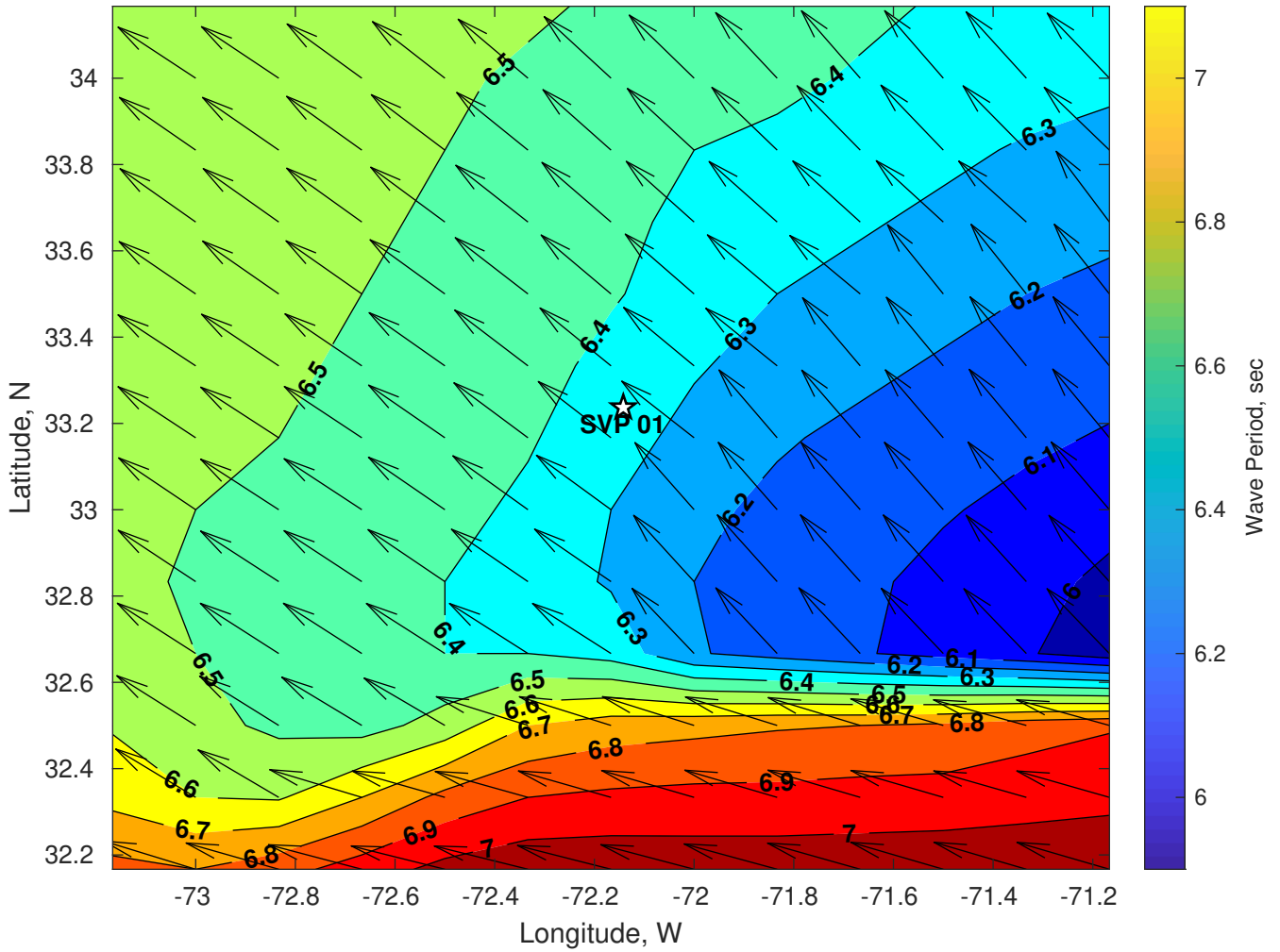
Wave Period (sec) for SVP 01 at 10-Jul-2024 06:00:00
