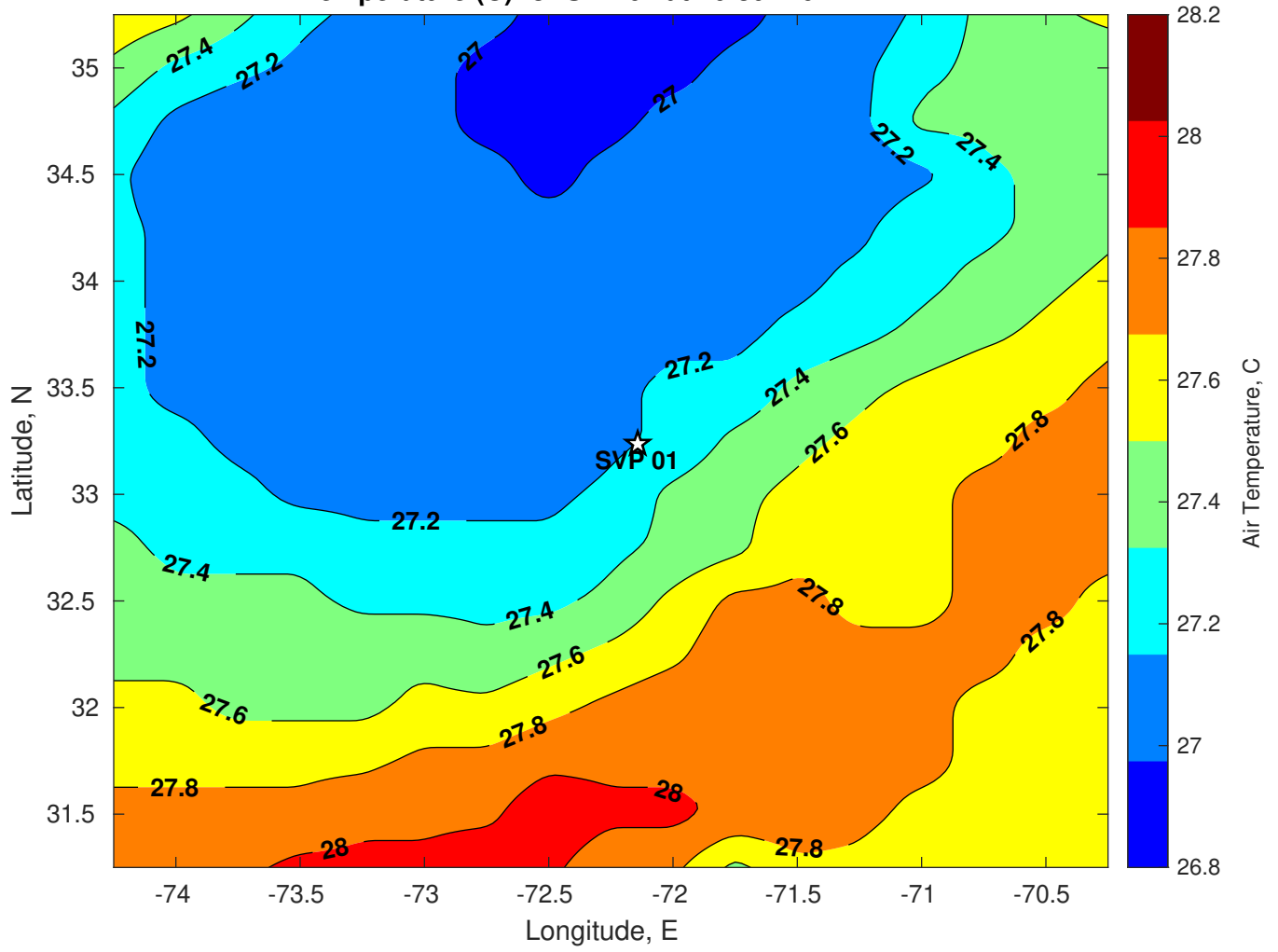
Air Temperature (C) for SVP 01 at 10-Jul-2024
