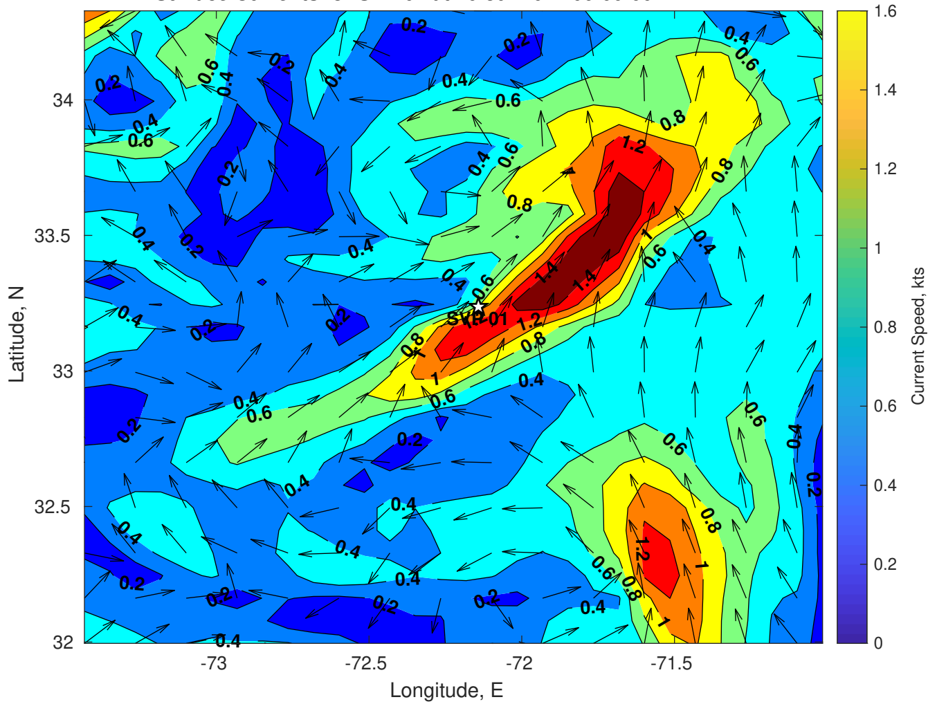
Surface Currents for SVP 01 at 10-Jul-2024 00:00:00
