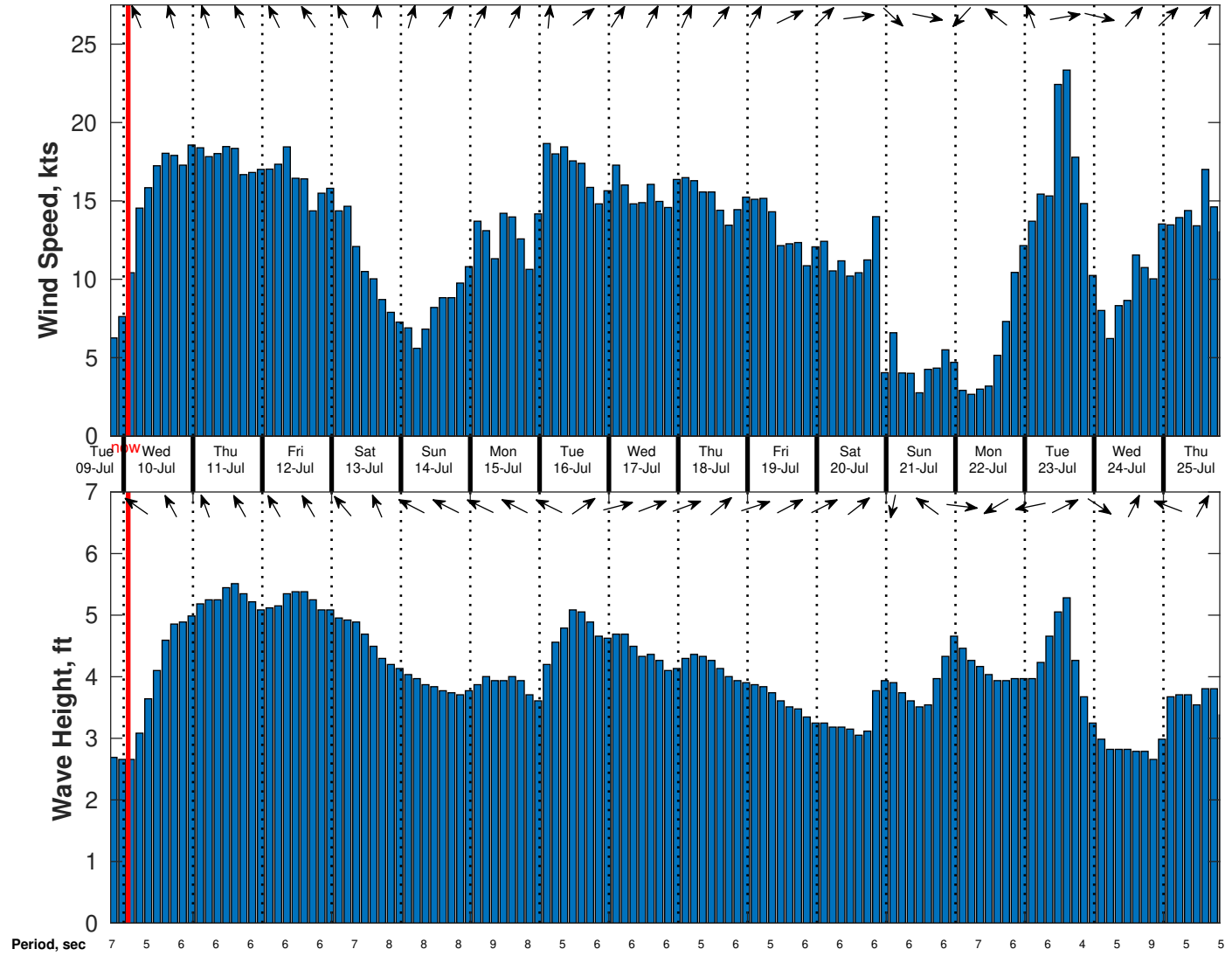
Wind & Wave Forecast for SVP 01 from 09-Jul-2024 19:00:00 to 25-Jul-2024 19:00:00
