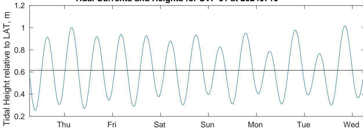
Tidal Currents and Heights for SVP 01 at 20240710
