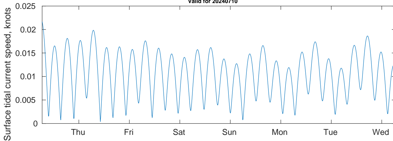
Tidal Currents and Heights for SVP 01 at 20240710
