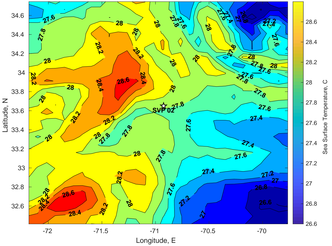
SST for SVP 02 at 10-Jul-2024 00:00:00
