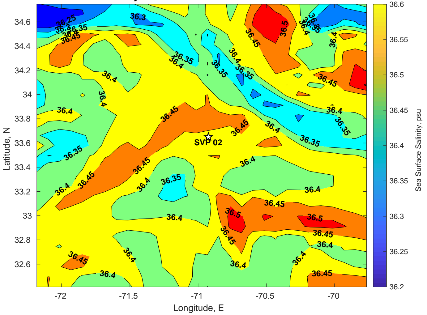
Surface Salinity for SVP 02 at 10-Jul-2024 00:00:00
