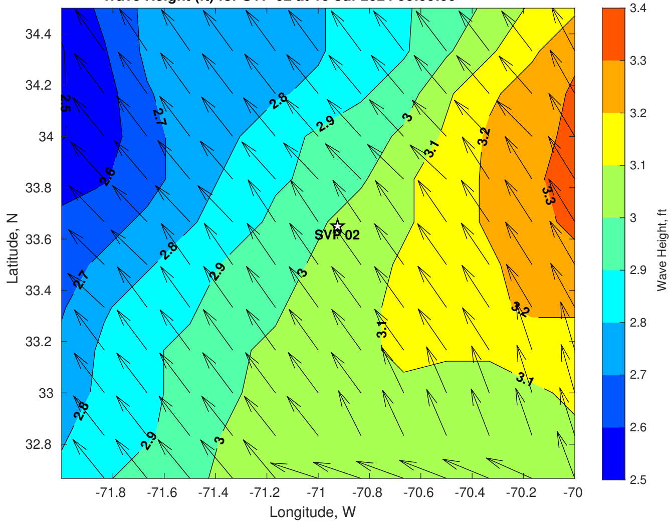
Wave Height (ft) for SVP 02 at 10-Jul-2024 06:00:00
