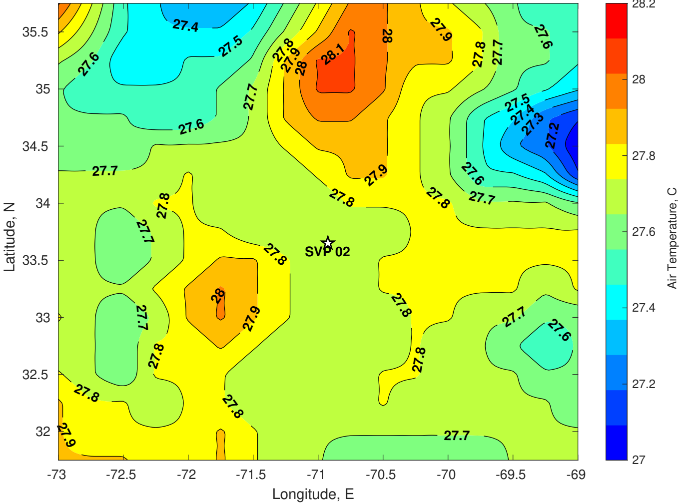
Air Temperature (C) for SVP 02 at 10-Jul-2024
