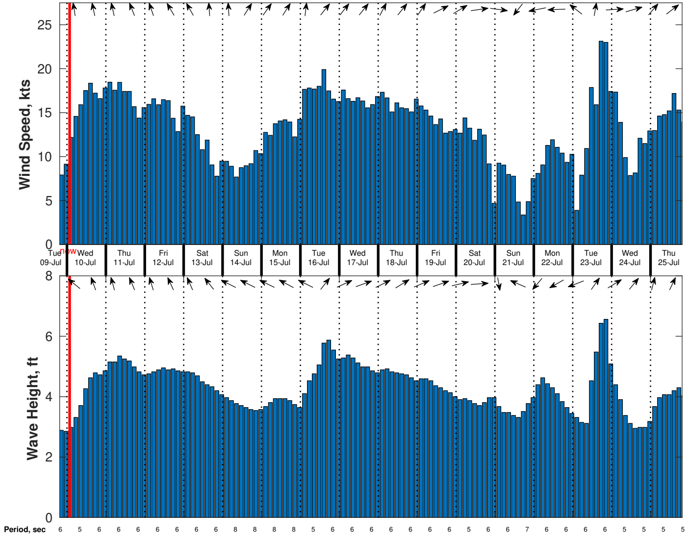
Wind & Wave Forecast for SVP 02 from 09-Jul-2024 19:00:00 to 25-Jul-2024 19:00:00
