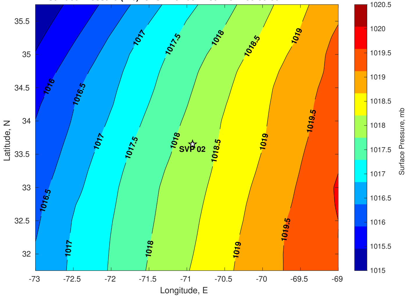
Surface Pressure (mb) for SVP 02 at 11-Jul-2024 00:00:00
