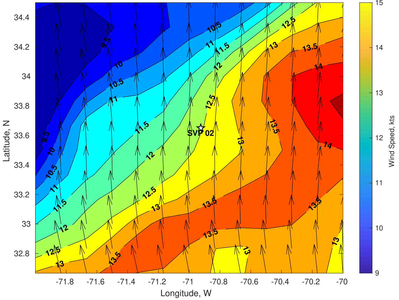
Winds (kts) for SVP 02 at 10-Jul-2024 06:00:00
