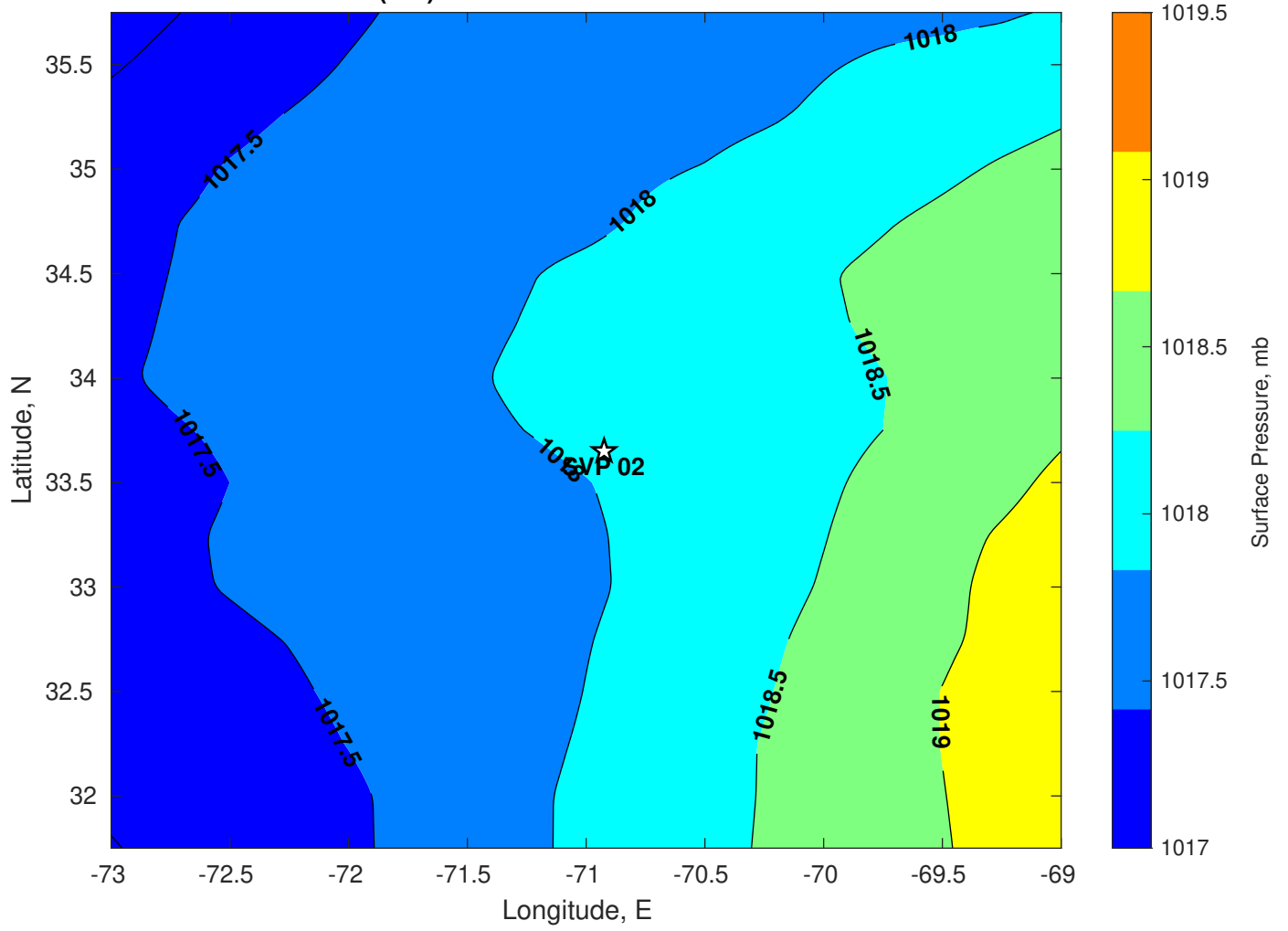
Surface Pressure (mb) for SVP 02 at 10-Jul-2024 00:00:00
