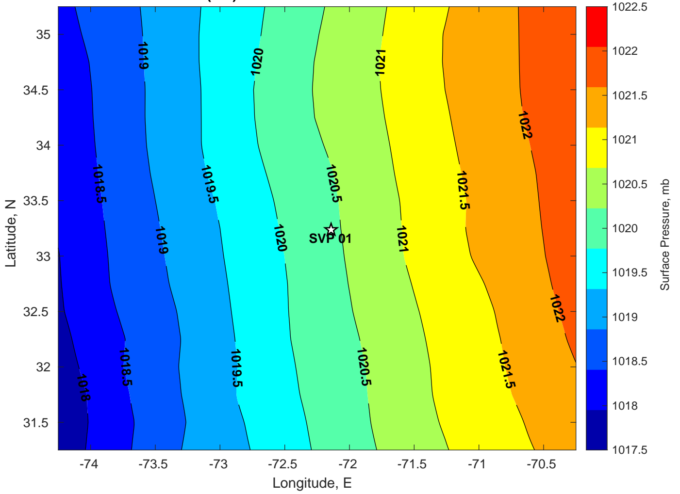
Surface Pressure (mb) for SVP 01 at 12-Jul-2024 00:00:00
