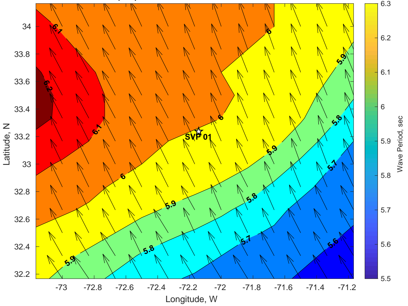
Wave Period (sec) for SVP 01 at 11-Jul-2024 06:00:00
