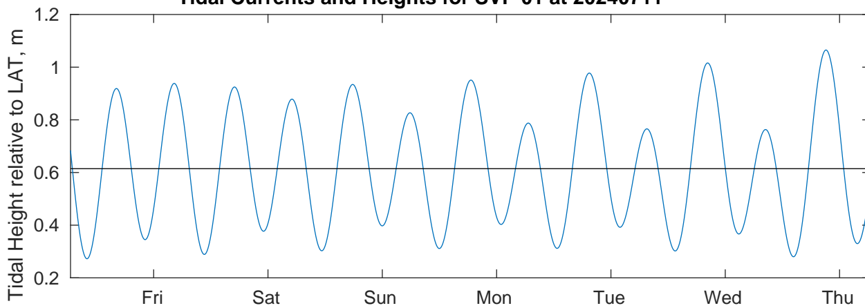
Tidal Currents and Heights for SVP 01 at 20240711
