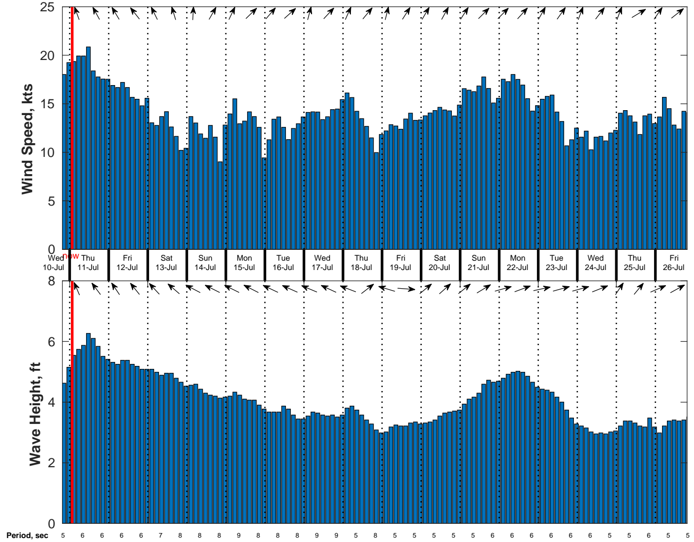
Wind & Wave Forecast for SVP 01 from 10-Jul-2024 19:00:00 to 26-Jul-2024 19:00:00
