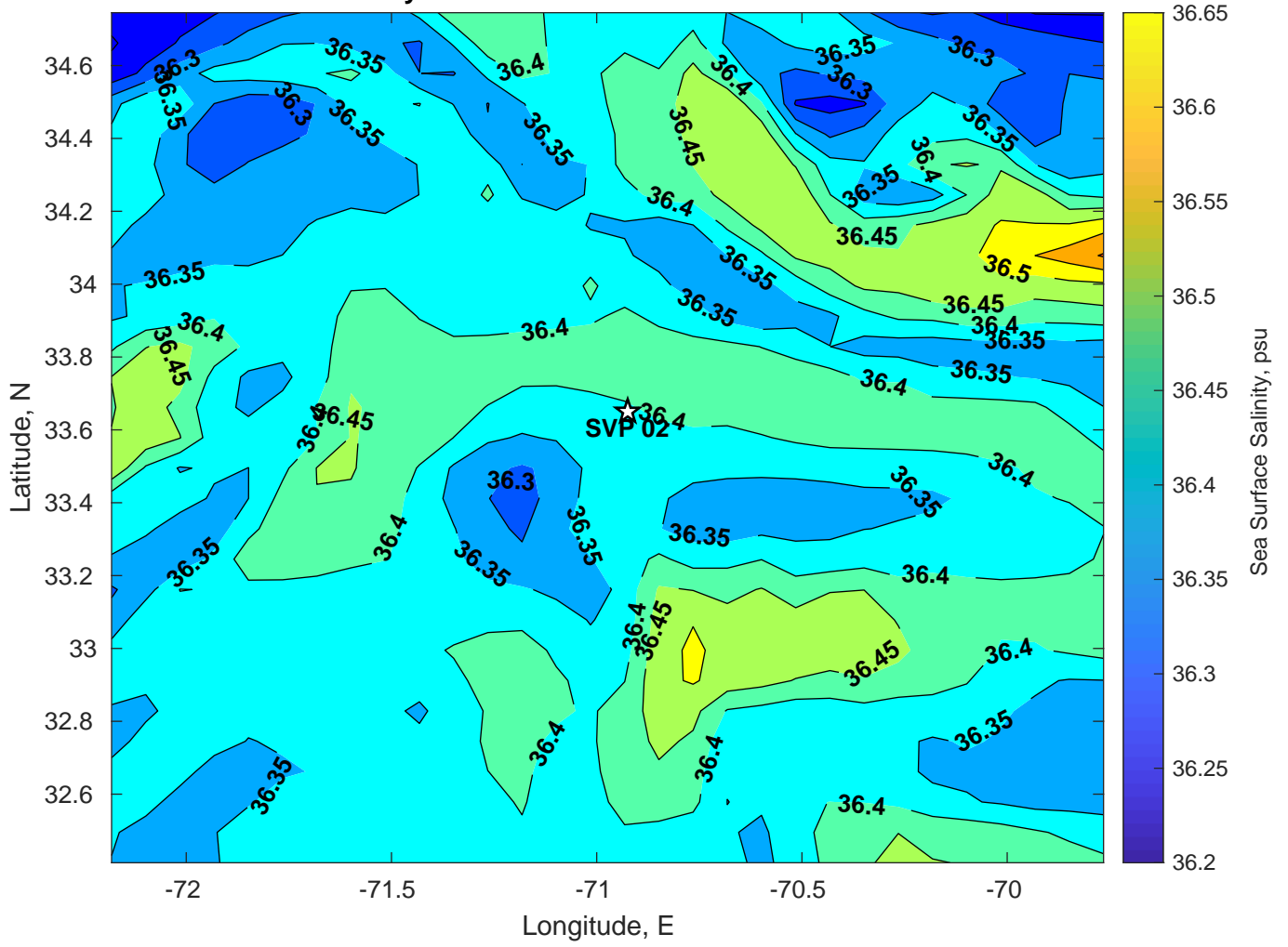
Surface Salinity for SVP 02 at 11-Jul-2024 00:00:00
