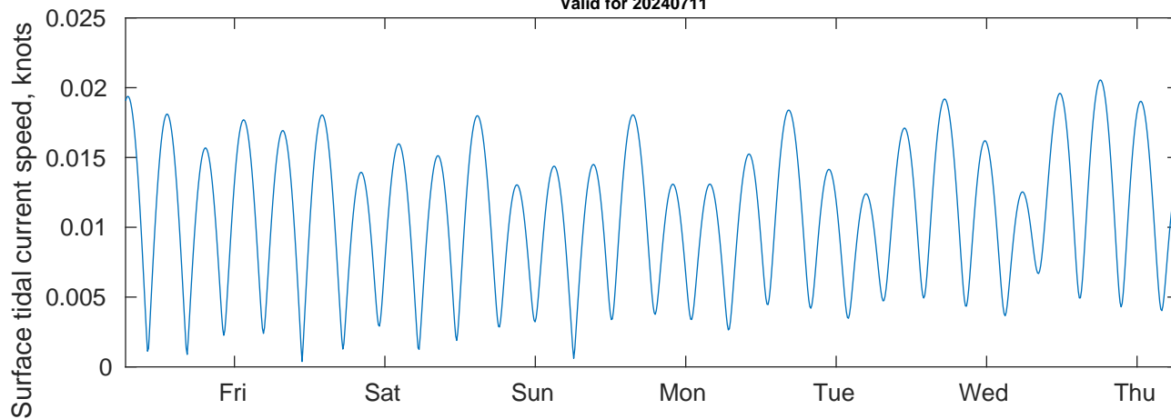
Tidal Currents and Heights for SVP 02 at 20240711
