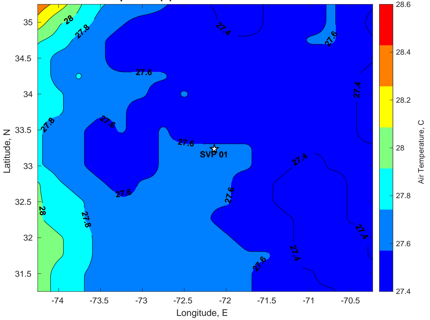
Air Temperature (C) for SVP 01 at 12-Jul-2024
