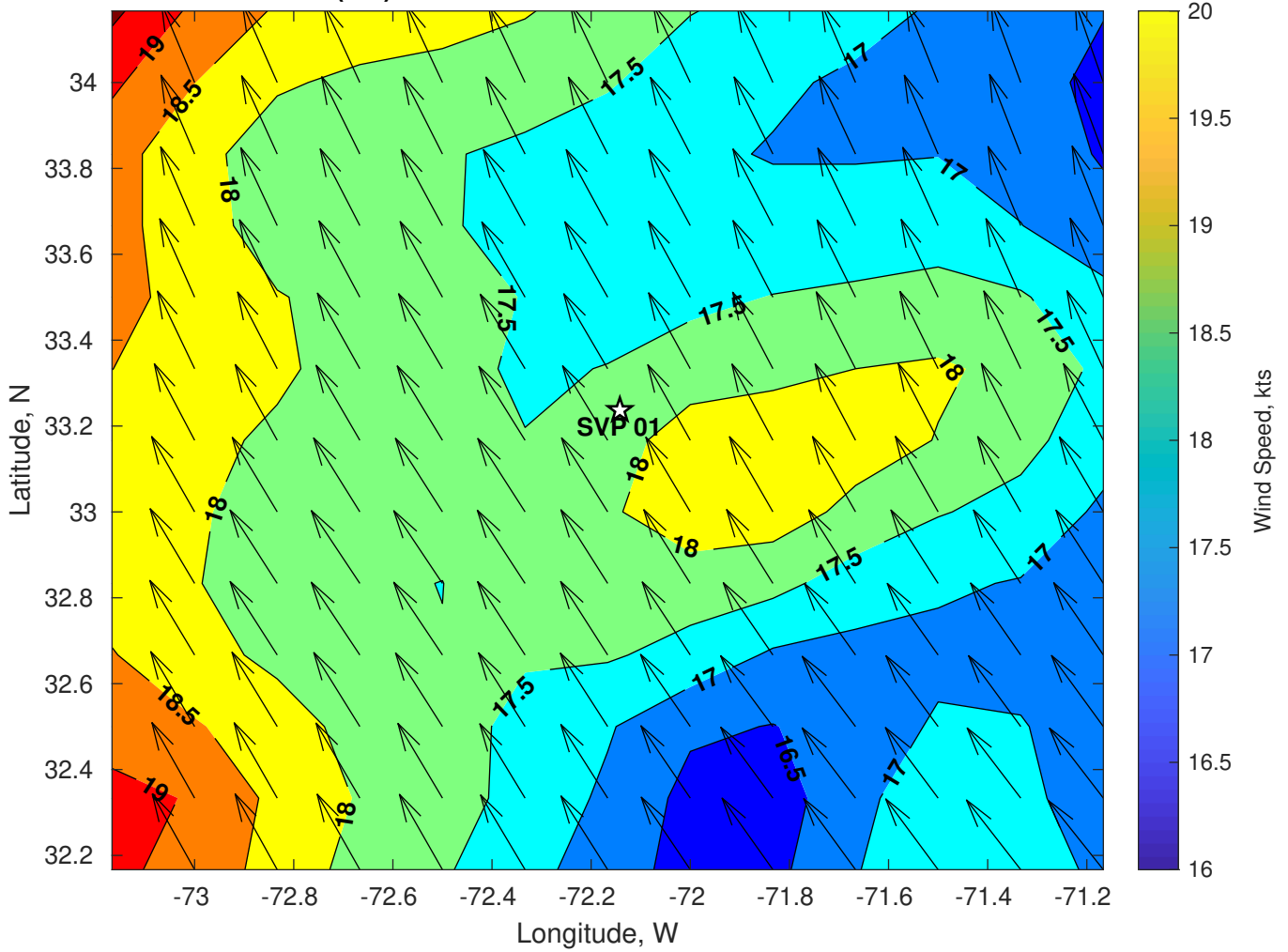
Winds (kts) for SVP 01 at 12-Jul-2024 06:00:00
