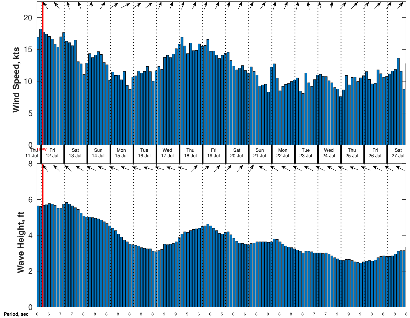
Wind & Wave Forecast for SVP 01 from 11-Jul-2024 19:00:00 to 27-Jul-2024 19:00:00
