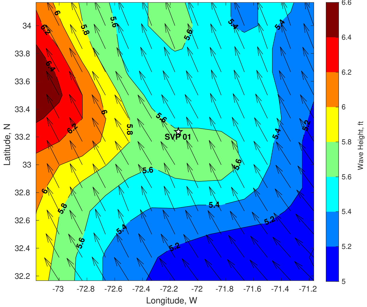
Wave Height (ft) for SVP 01 at 12-Jul-2024 06:00:00
