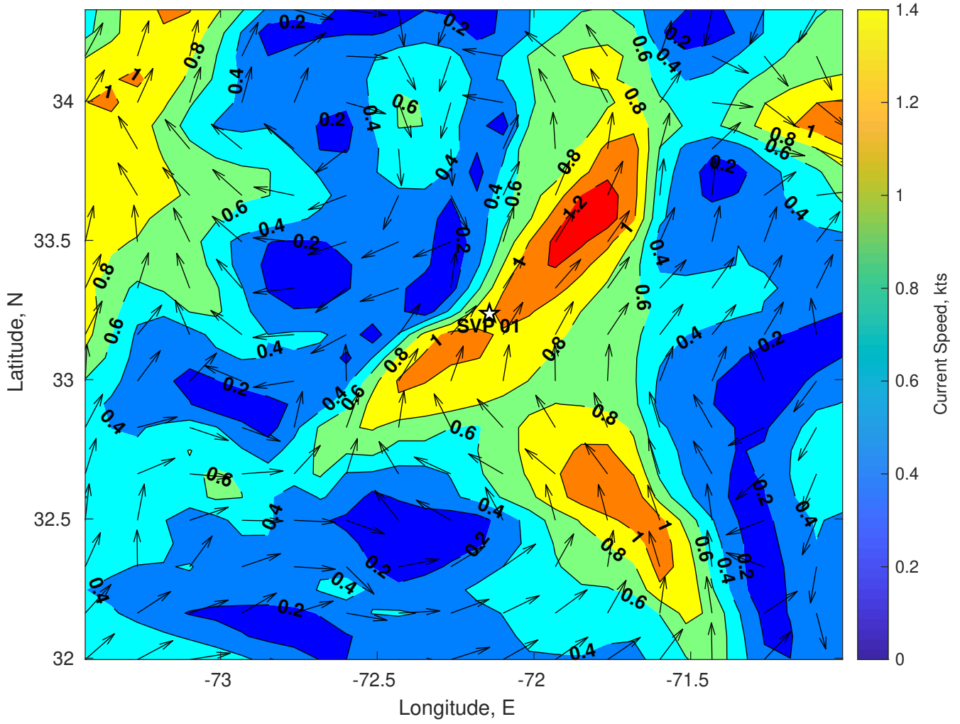
Surface Currents for SVP 01 at 12-Jul-2024 00:00:00
