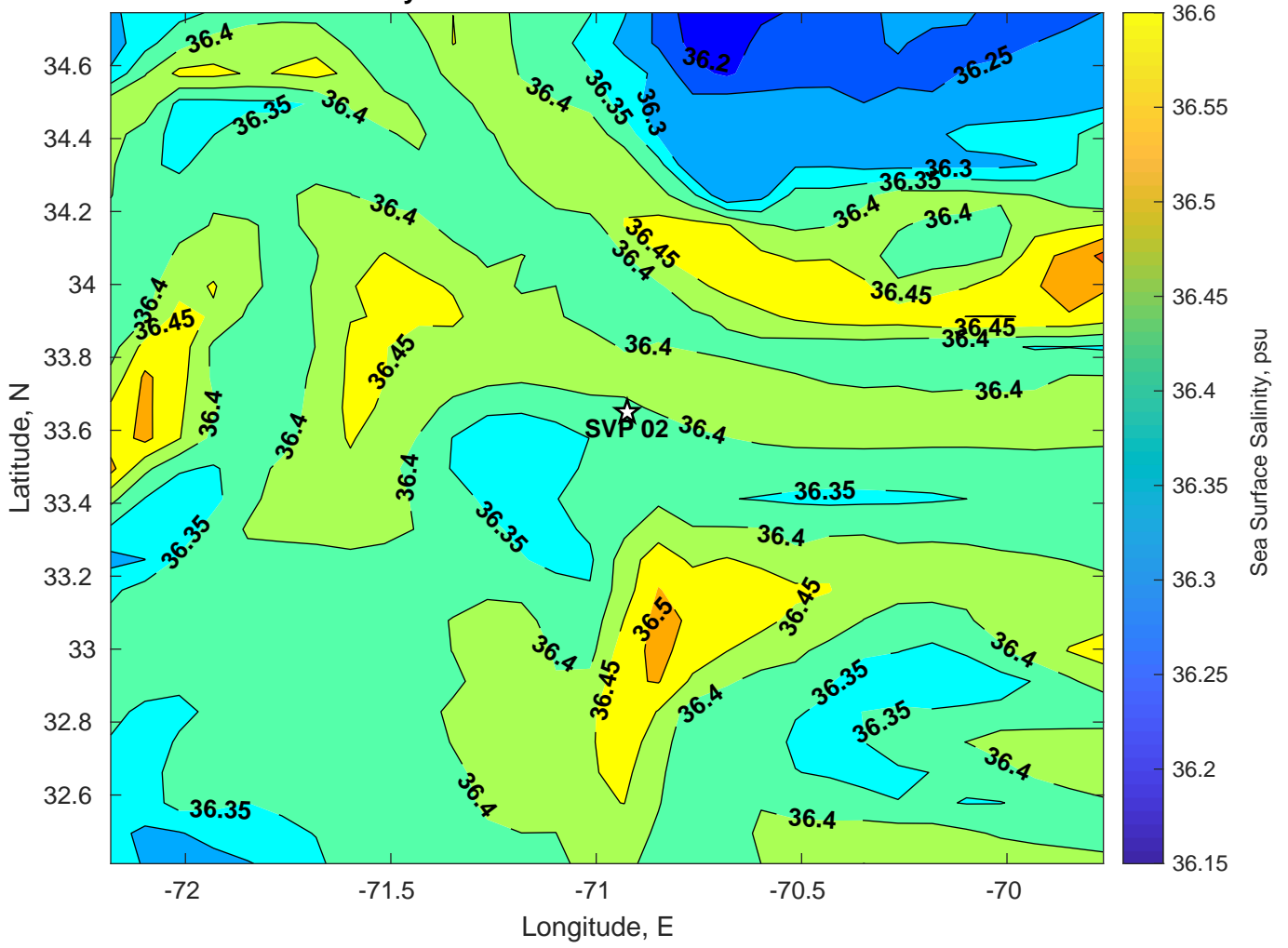
Surface Salinity for SVP 02 at 12-Jul-2024 00:00:00
