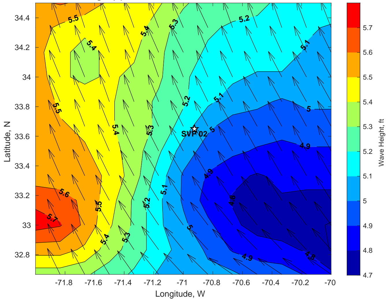
Wave Height (ft) for SVP 02 at 12-Jul-2024 06:00:00
