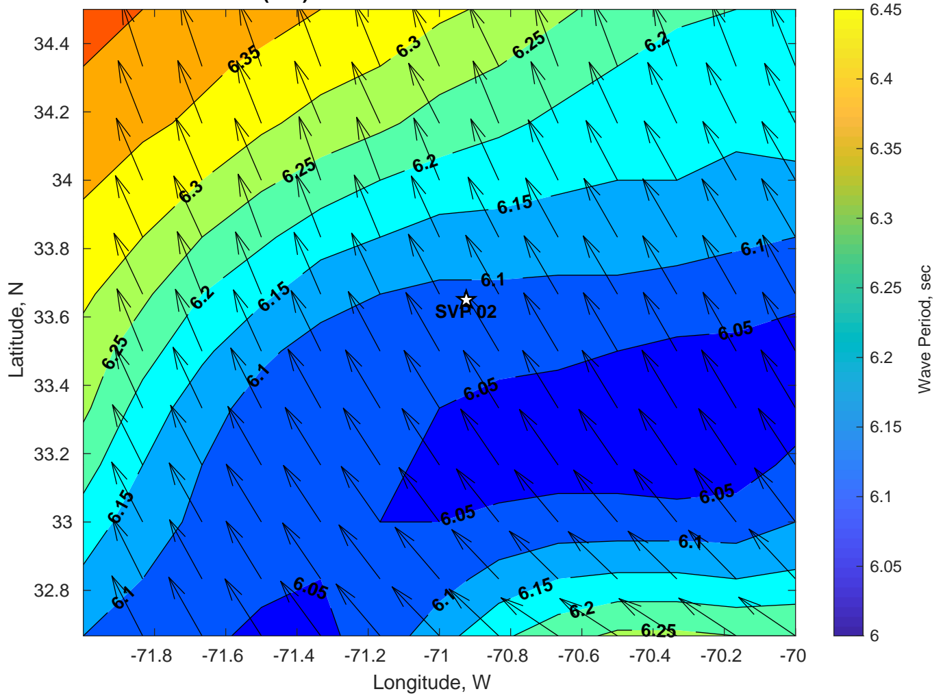
Wave Period (sec) for SVP 02 at 12-Jul-2024 06:00:00
