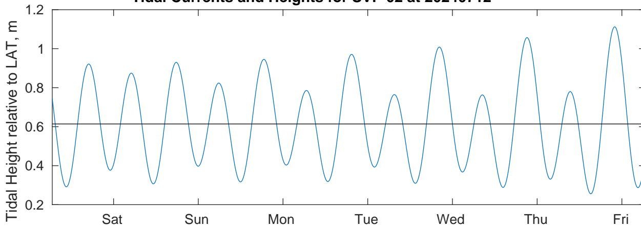
Tidal Currents and Heights for SVP 02 at 20240712
