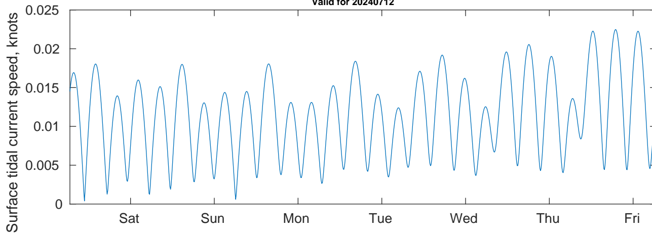
Tidal Currents and Heights for SVP 02 at 20240712
