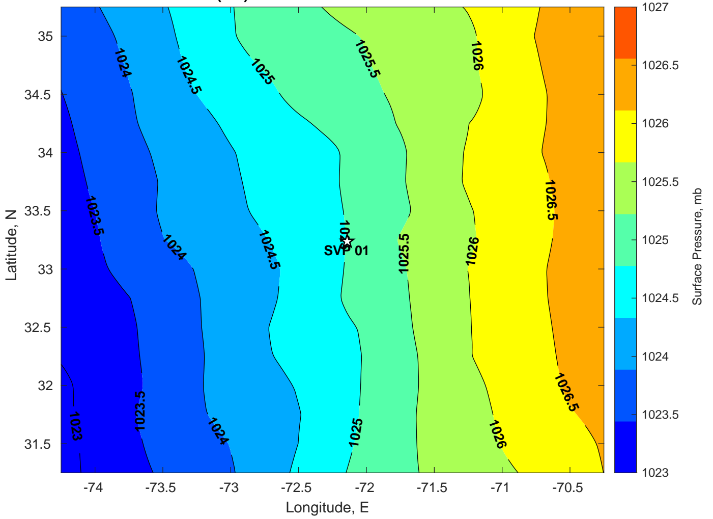
Surface Pressure (mb) for SVP 01 at 13-Jul-2024 00:00:00
