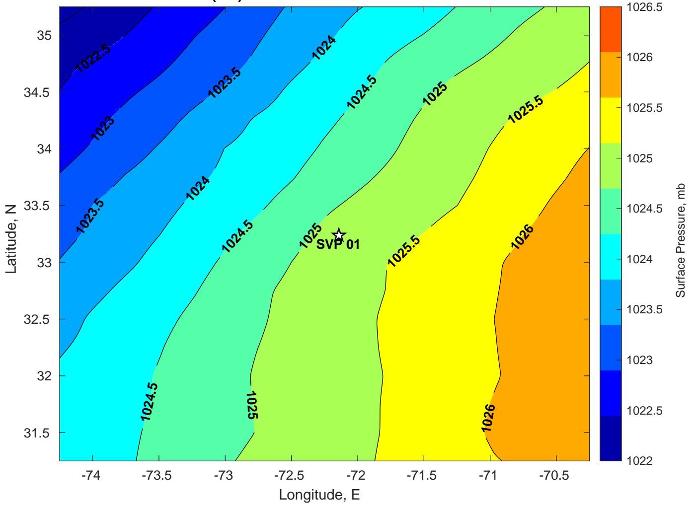
Surface Pressure (mb) for SVP 01 at 14-Jul-2024 00:00:00
