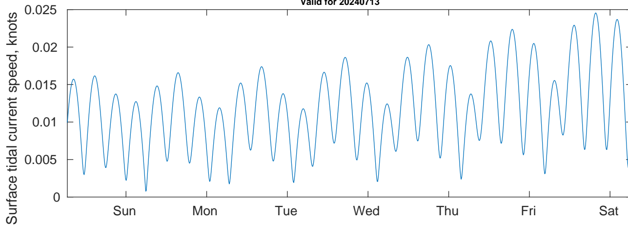
Tidal Currents and Heights for SVP 01 at 20240713
