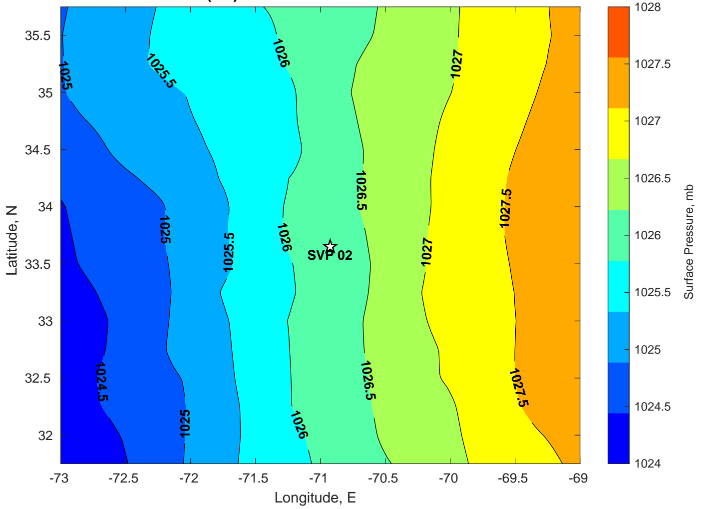
Surface Pressure (mb) for SVP 02 at 13-Jul-2024 00:00:00
