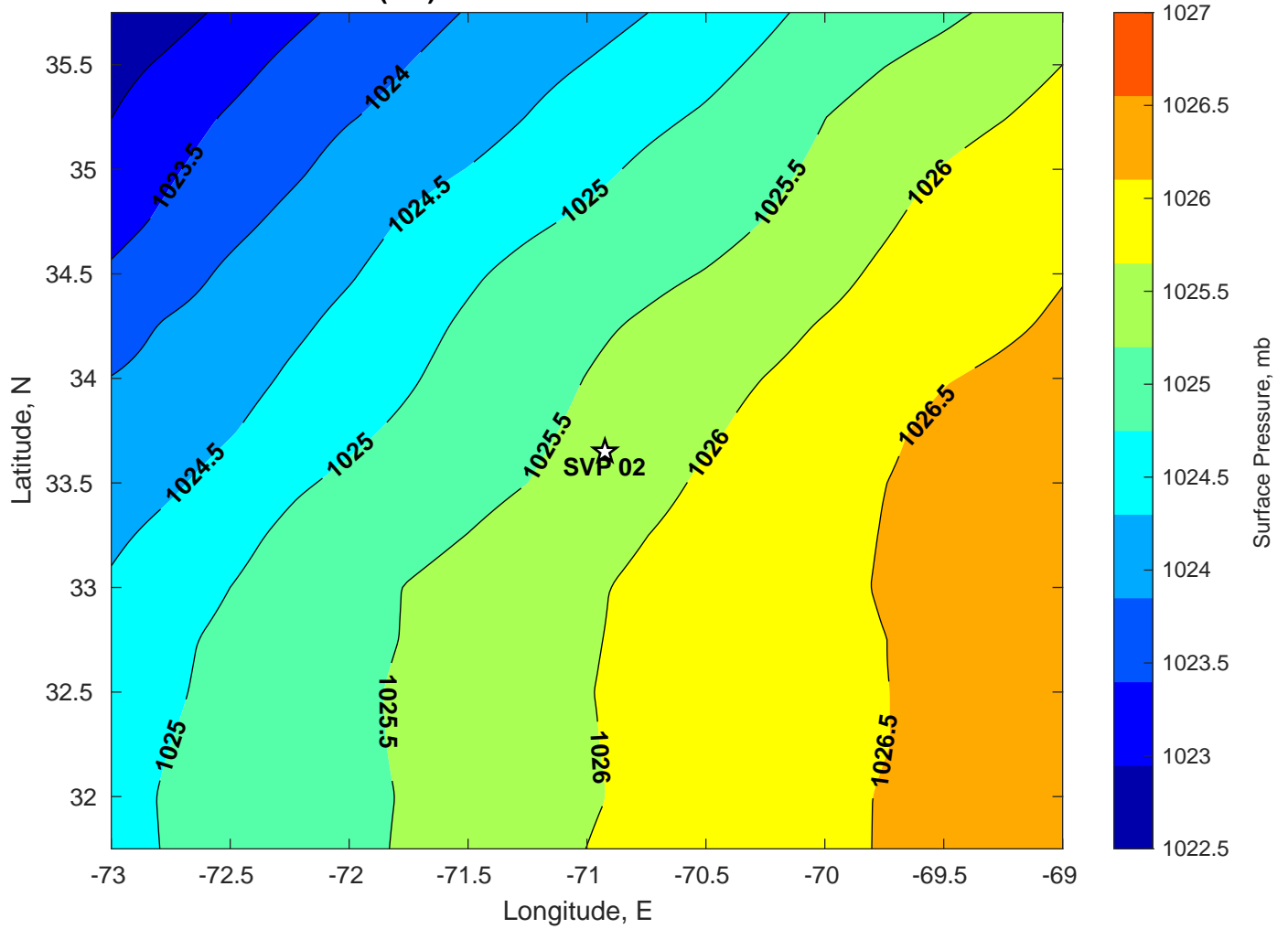
Surface Pressure (mb) for SVP 02 at 14-Jul-2024 00:00:00
